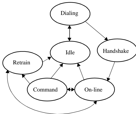
Figure 4. Modem State Diagram
