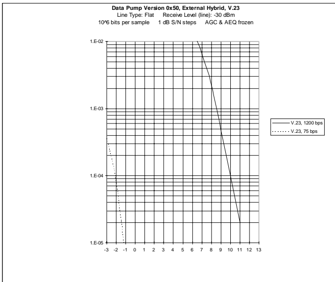
Figure 6. Typical Performance Data
