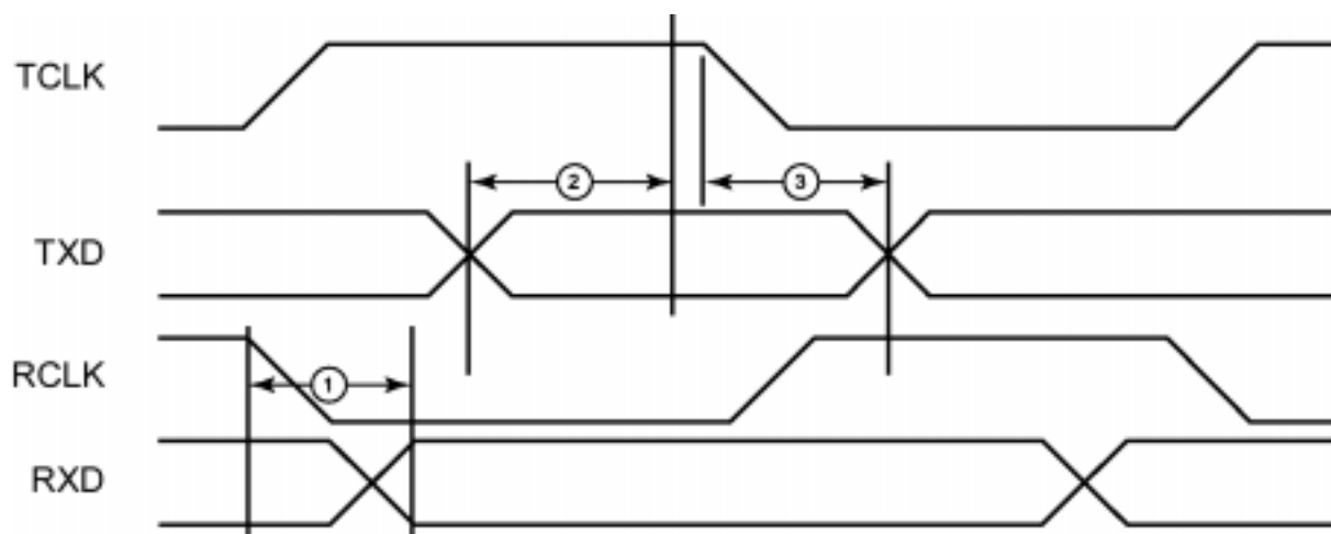
Figure 9. Serial Port Timing Diagram
