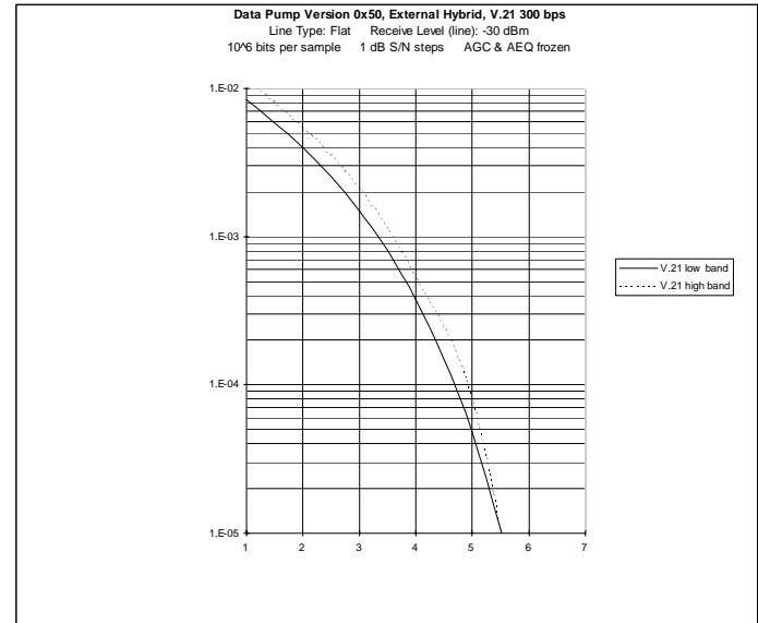
Figure 6. Typical Performance Data
