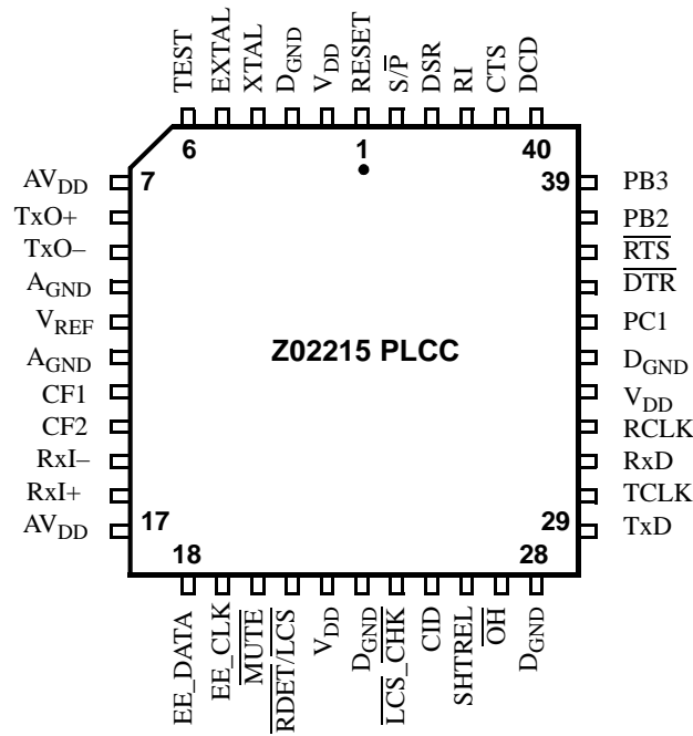
Figure 2. Z02215 44-Lead PLCC Pin Identification
