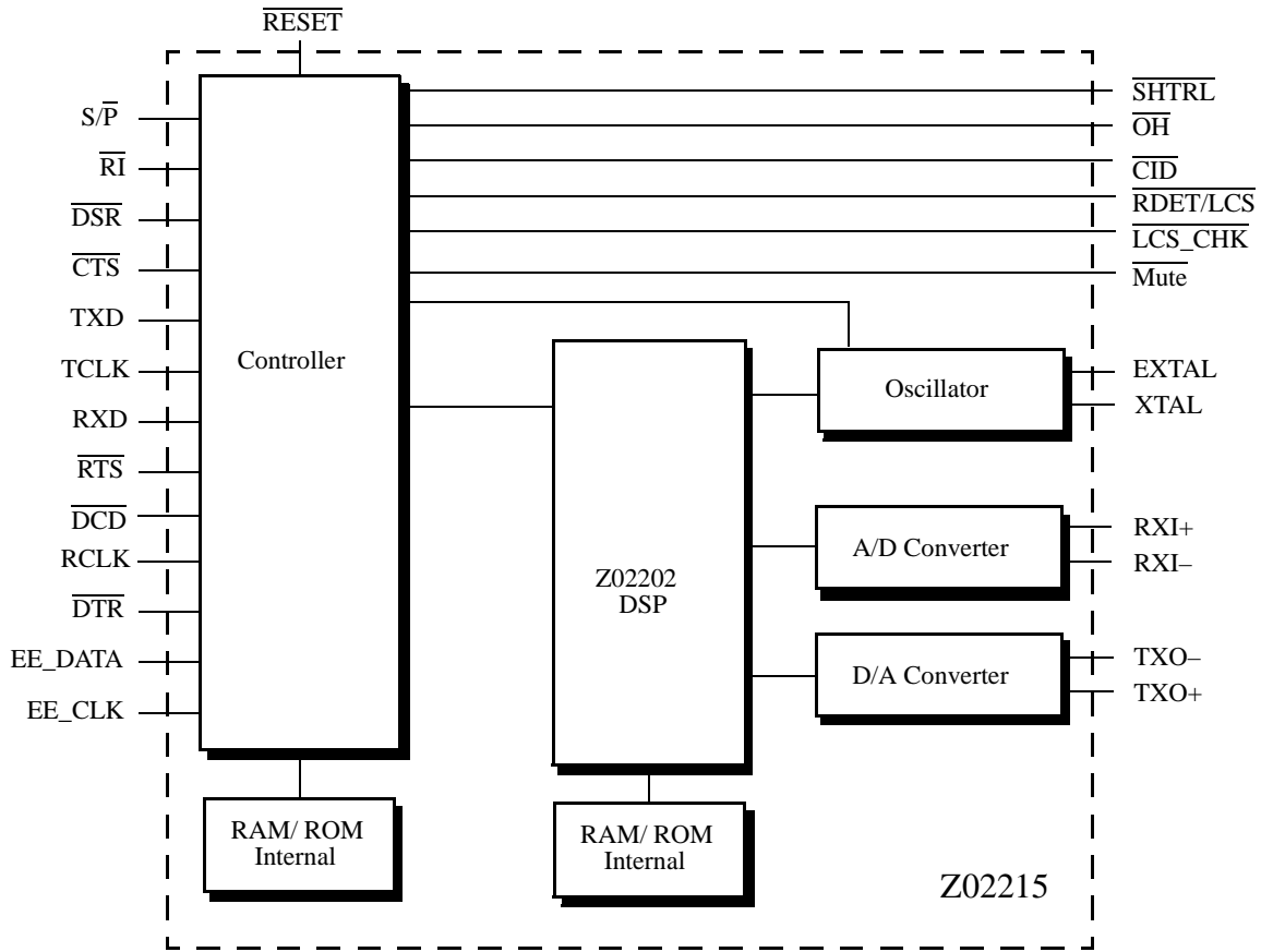
Figure 1. Z02215 Block Diagram
