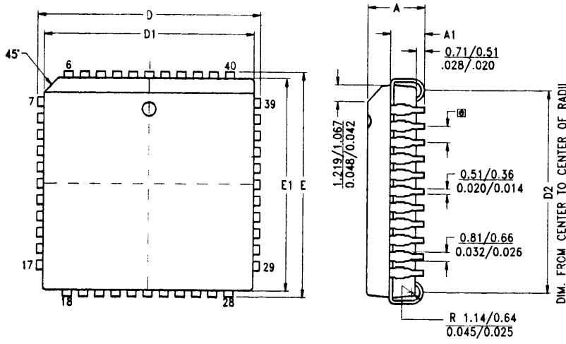
Figure 10. 44-Lead PLCC Package Diagram
