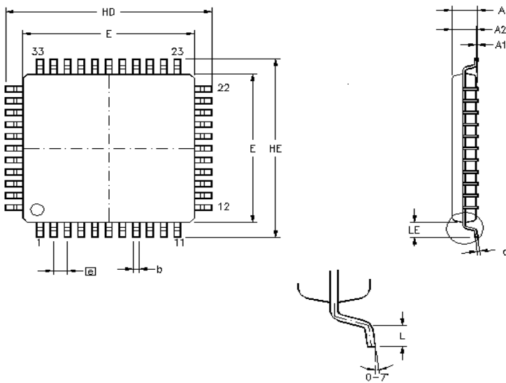
Figure 11. 44-Lead VQFP Package Diagram
