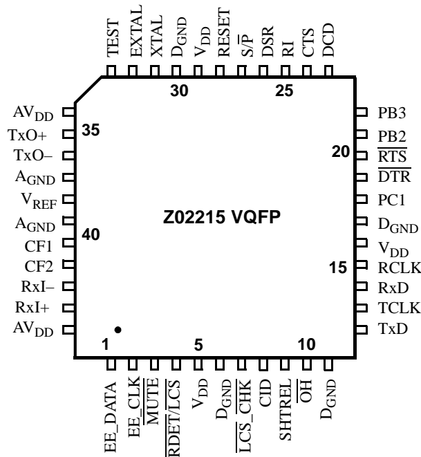
Figure 3. Z02215 44-Lead VQFP Pin Identification
