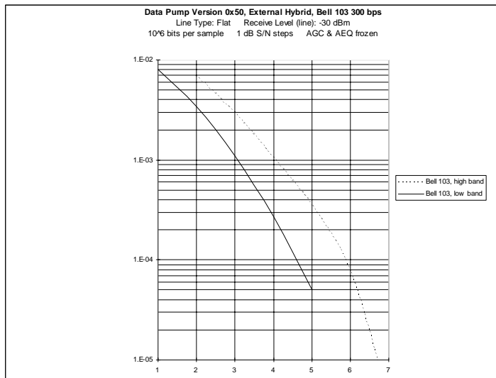
Figure 6 (Continued). Typical Performance Data
