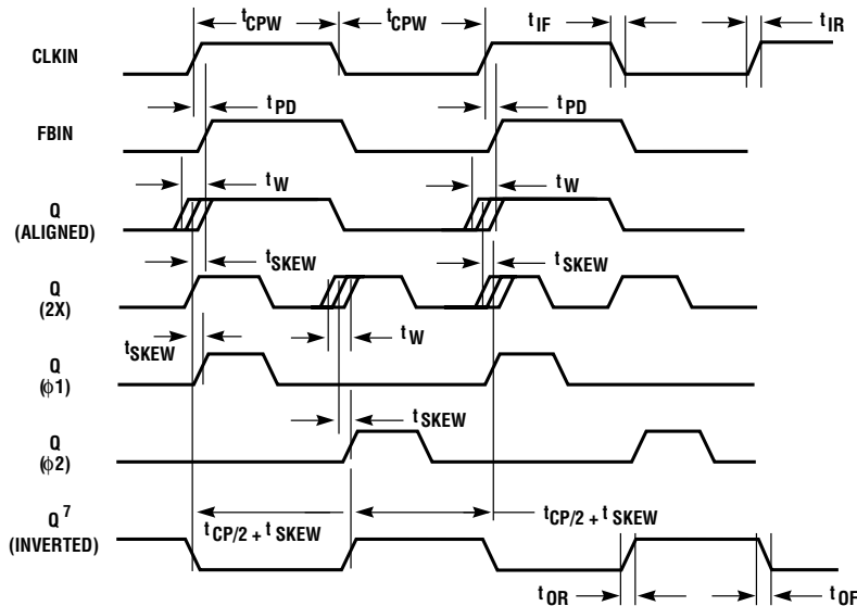
Figure 7. Switching Waveforms
