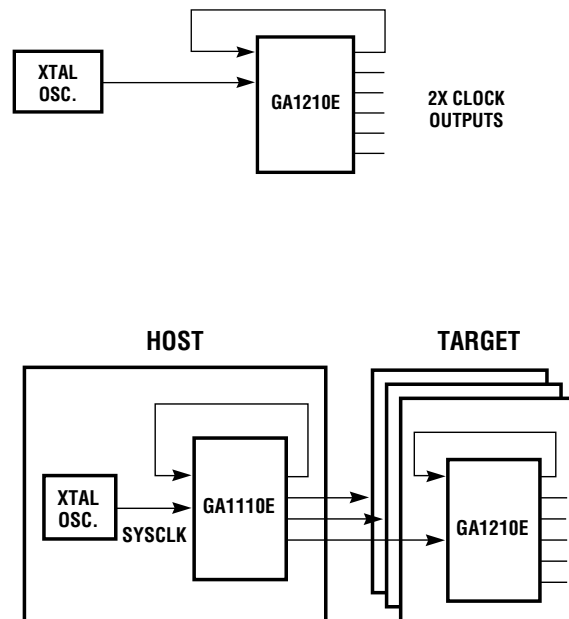
Figure 5. Typical Applications
