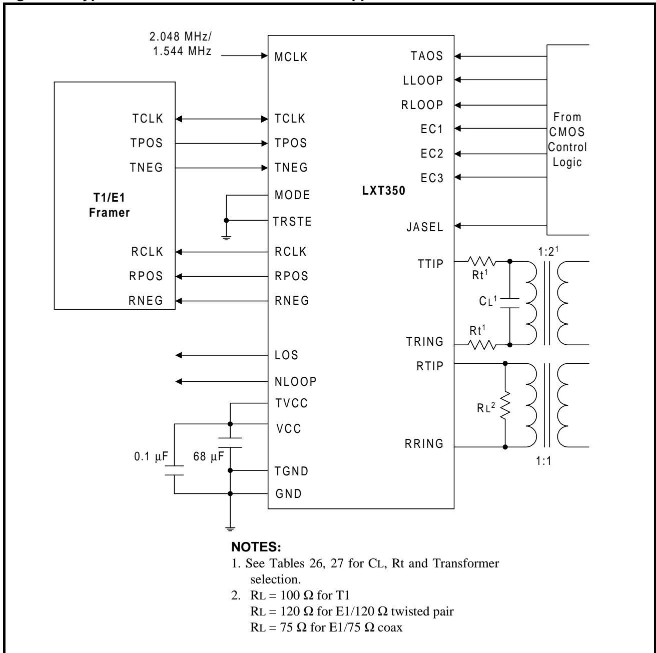
Figure 13: Typical T1/E1 LXT350 Hardware Mode Application
