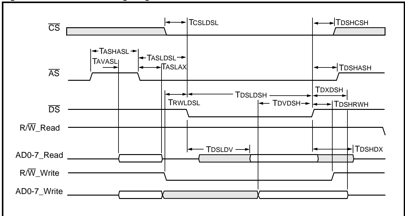
Figure 23: LXT351 I/O Timing Diagram for Motorola Address/Data Bus
