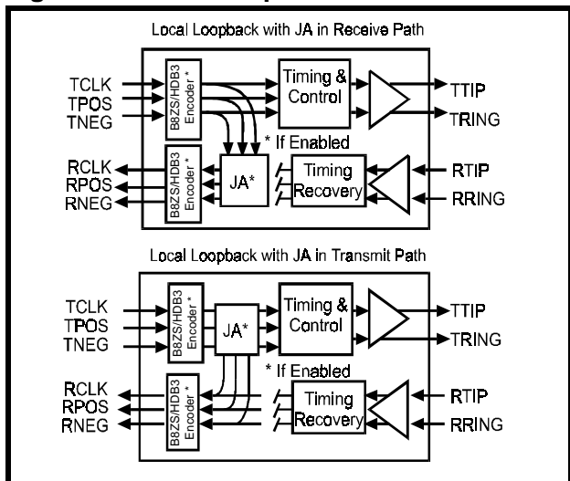
Figure 6: Local Loopback
