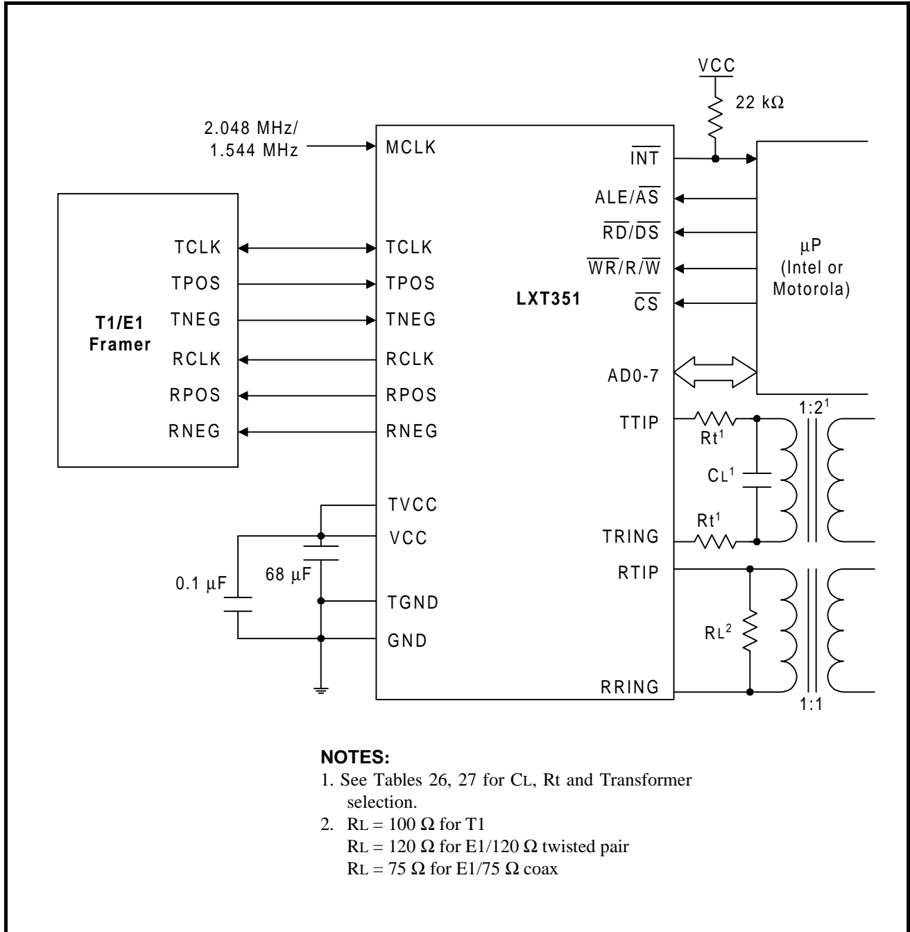
Figure 15: Typical T1/E1 LXT351 Application
