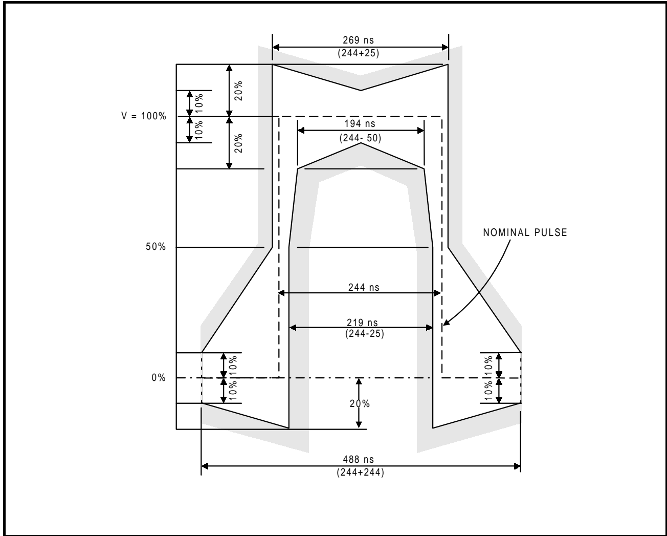
Figure 16: 2.048 Mbps E1 Pulse (See Table 35)
