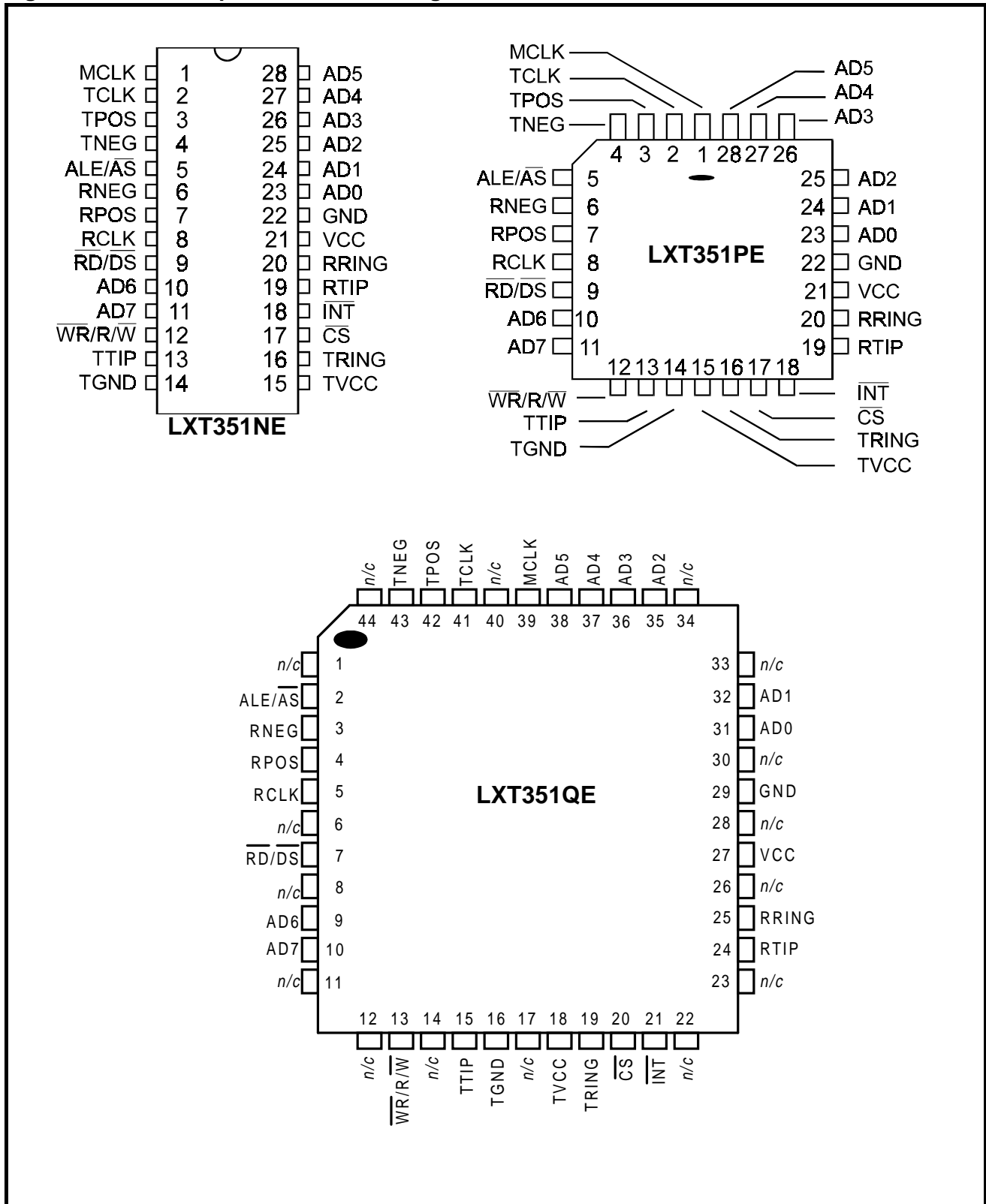
Figure 2: LXT351 Bipolar Mode Pin Assignments
