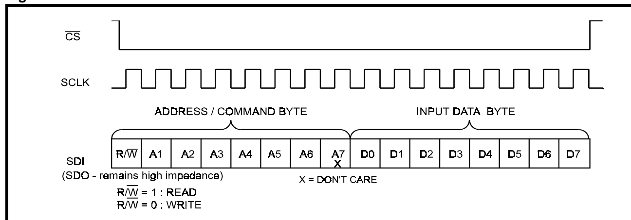
Figure 12: LXT350 Serial Interface Data Structure
