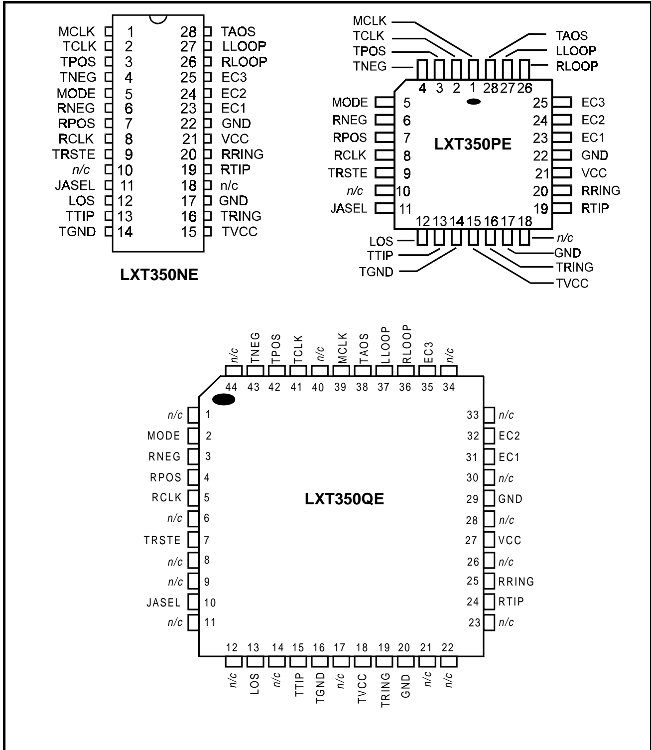
Figure 1: LXT350 Hardware Controlled Bipolar Mode Pin Assignments
