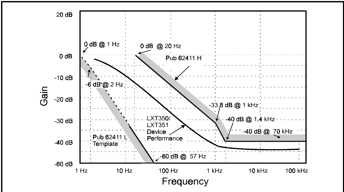
Figure 26: Typical T1 Jitter Transfer Performance
