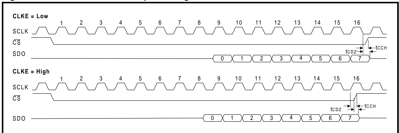
Figure 21: LXT350 Serial Data Output Timing
