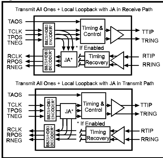
Figure 6: Local Loopback
