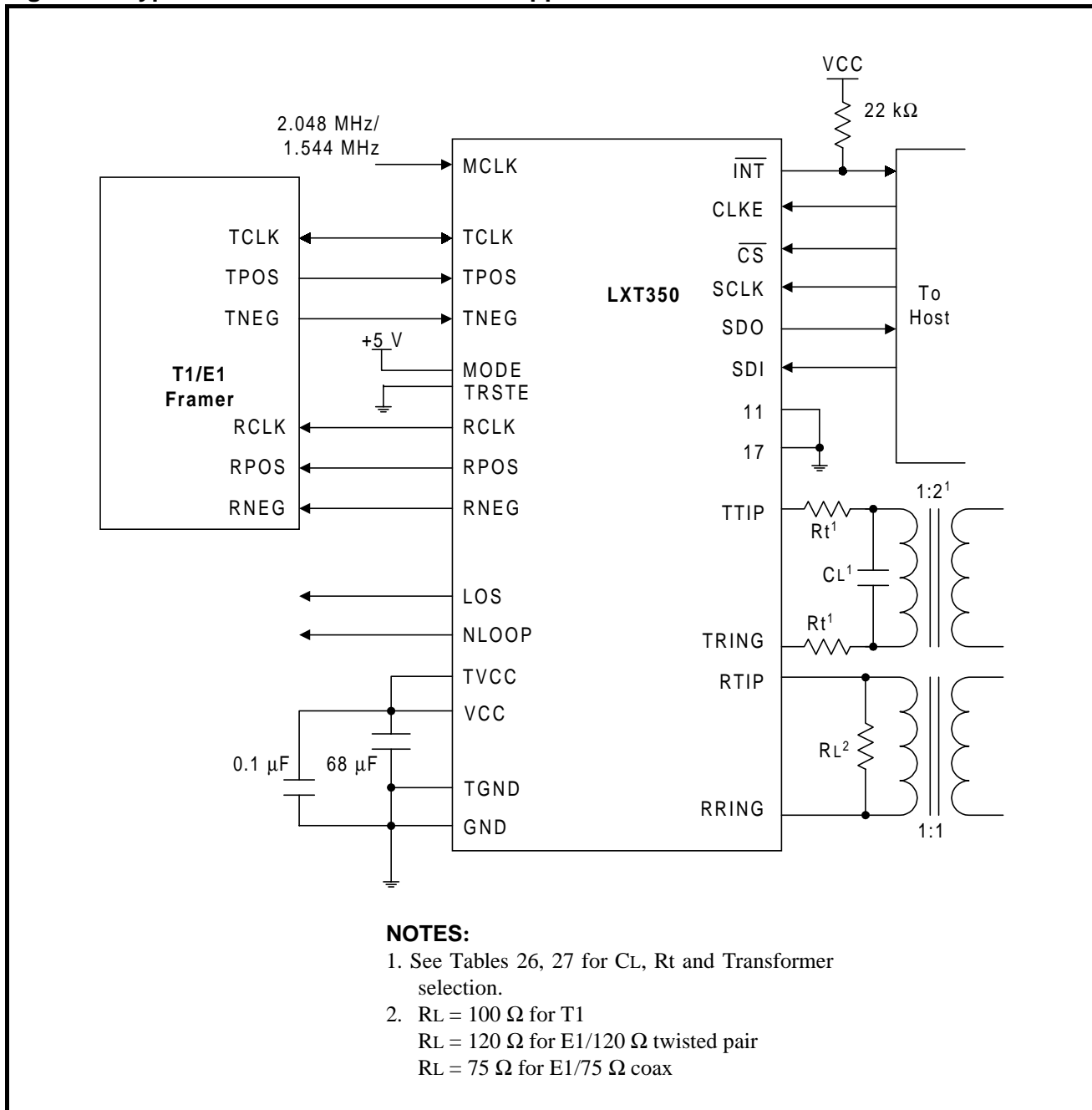
Figure 14: Typical T1/E1 LXT350 Host Mode Application
