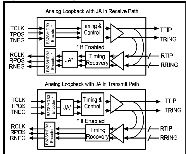
Figure 7: Analog Loopback
