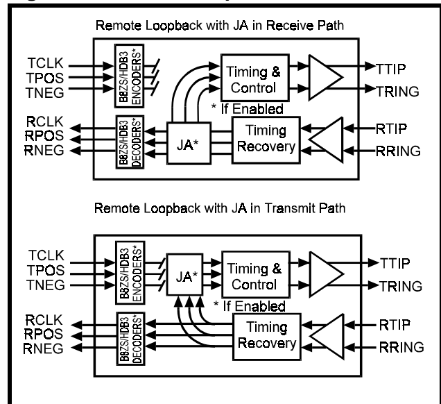
Figure 8: Remote Loopback
