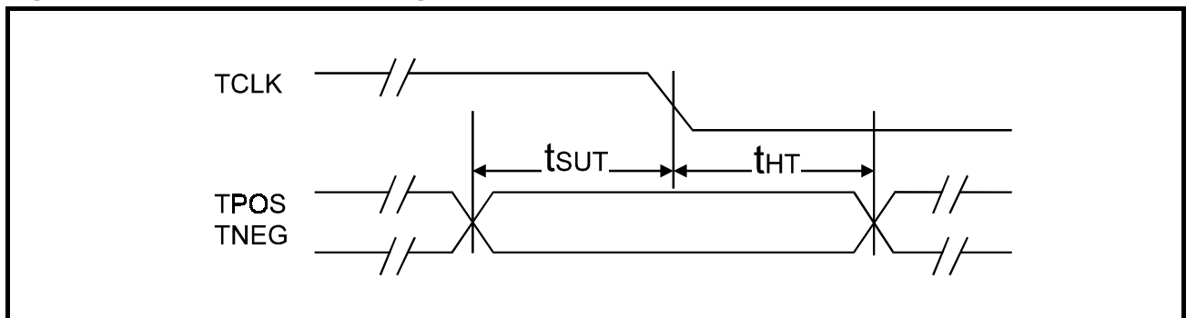
Figure 18: Transmit Clock Timing
