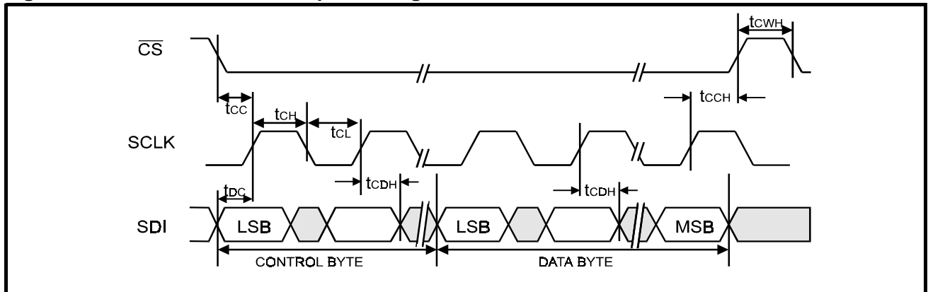
Figure 20: LXT350 Serial Data Input Timing
