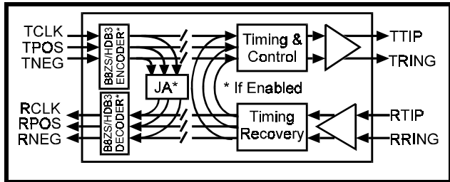
Figure 9: Dual Loopback
