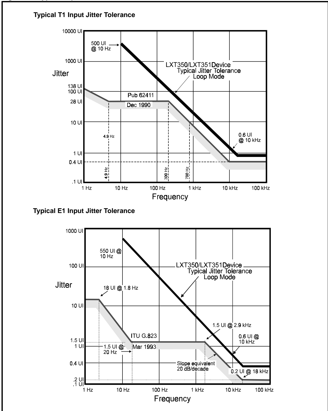
Figure 24: Typical Input Jitter Tolerance
