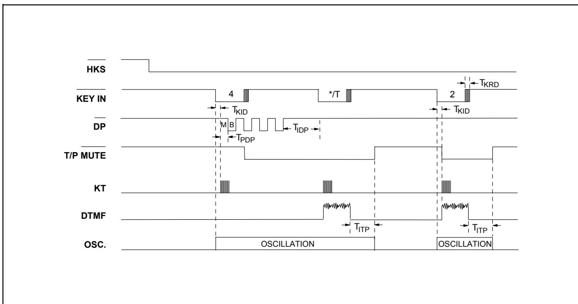
Figure 5(b). Pulse-to-tone Timing Diagram (W91534AN only)
