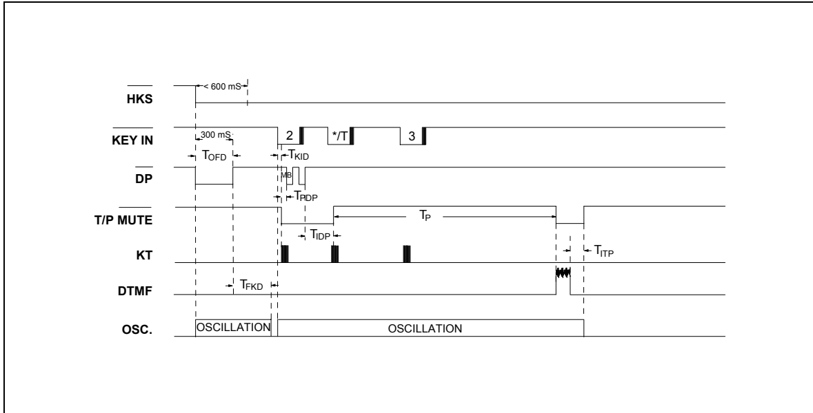
Figure 5(a). Pulse-to-tone Timing Diagram (except W91534AN)
