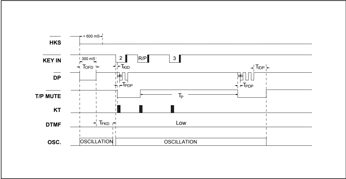
Figure 4. Pause Function Timing Diagram
