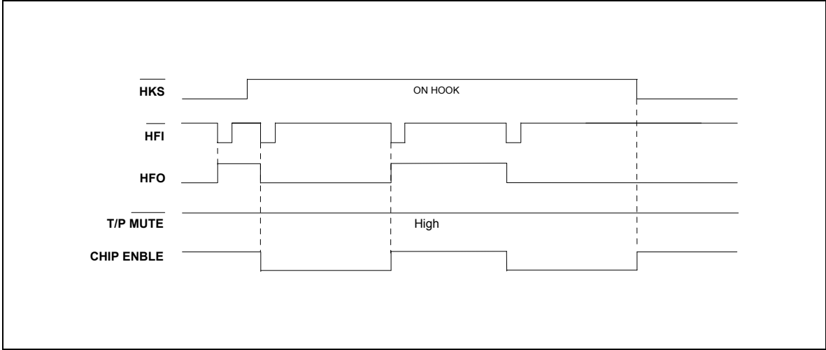
Figure 3. Handfree Timing Diagram
