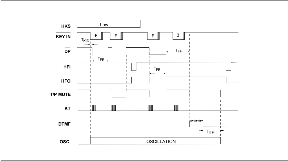
Figure 6. Flash Timing Diagram
