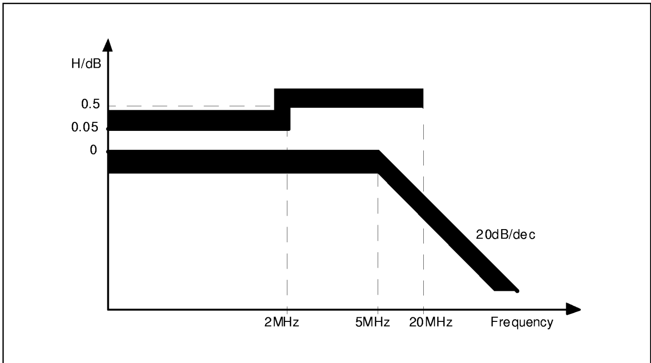
Figure 3 Jitter Transfer Function
