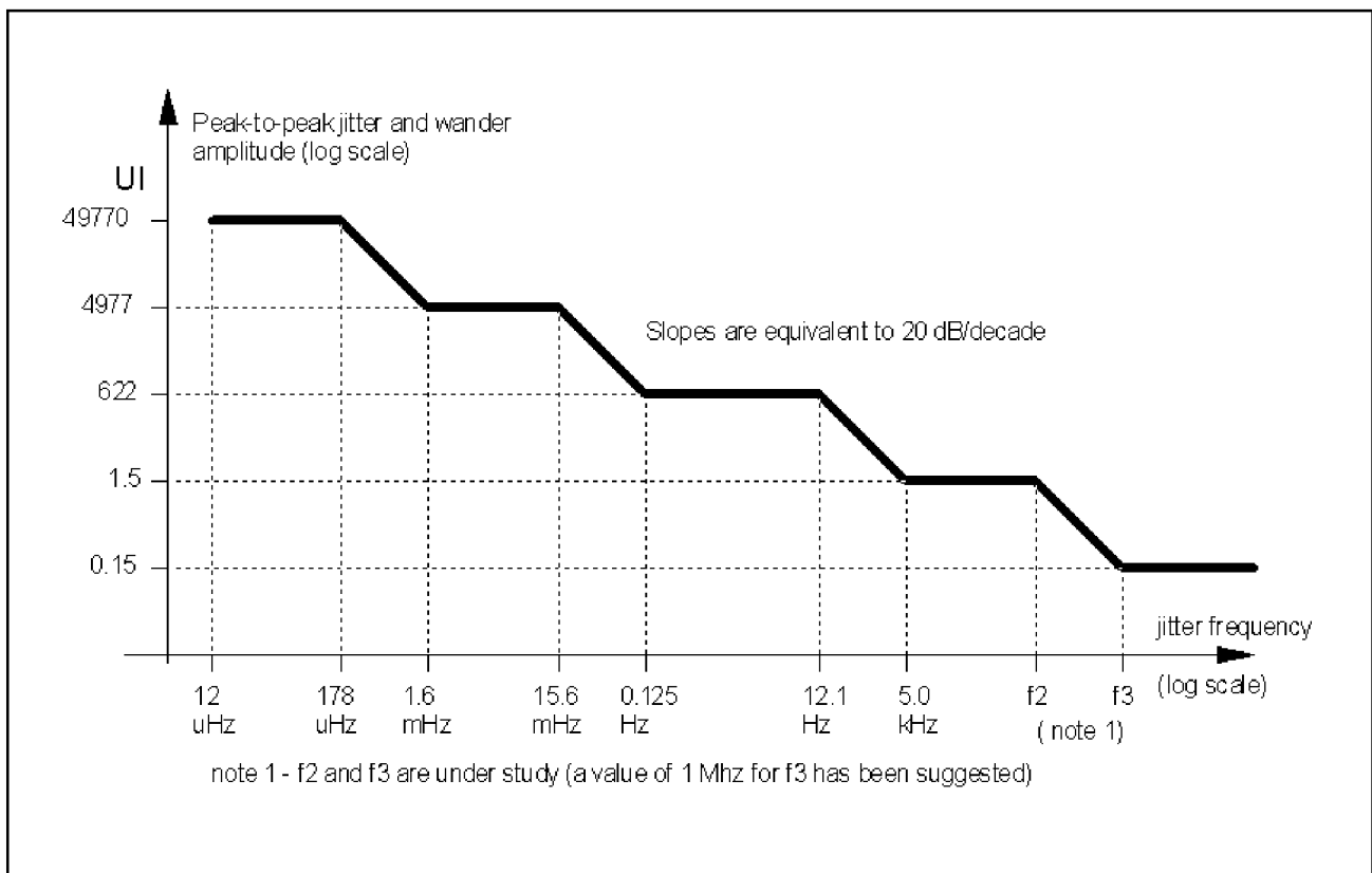
Figure 2 Lower Limit of Maximum Tolerable Jitter and Wander
