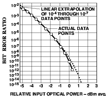
Figure 3. Relative Input Optical Power—dBm Avg.
