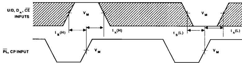
Waveform 6. Waveforms Showing Setup Time and Hold Time for D n to PL, U/D to CP and CE to CP
