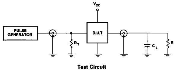
Test Circuit
