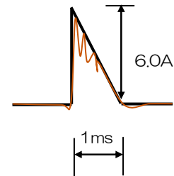
Fig. C : Inrush current waveform
