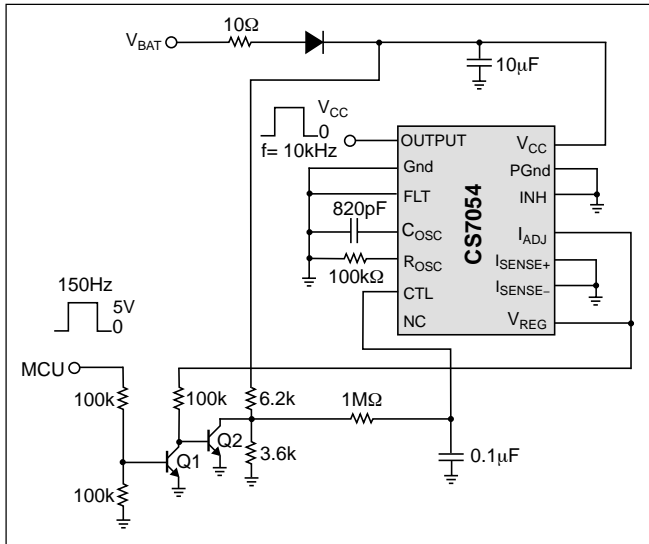
Figure 2: Frequency Converter
