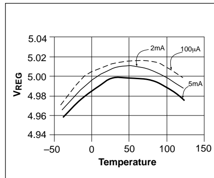
V_{REG} vs. Temperature @ V_{CC} = 12V
