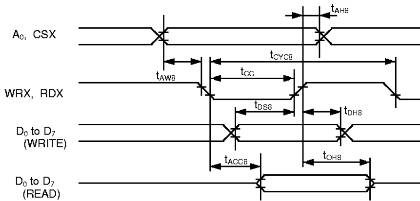
Figure 2 Read/write timing with 80 family MPU
