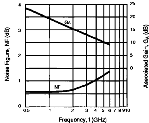
NOISE FIGURE & ASSOCIATED GAIN vs. FREQUENCY V CE = 3 V, I D = 20 mA
