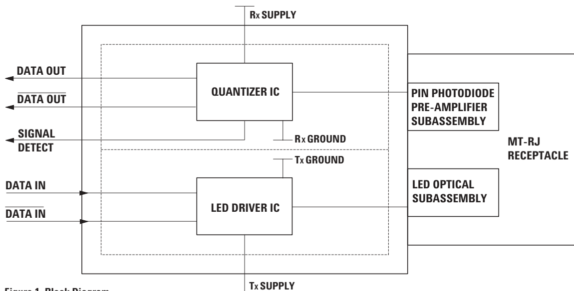
Figure 1. Block Diagram.
