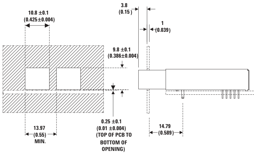
Figure 10. Recommended Panel Mounting
