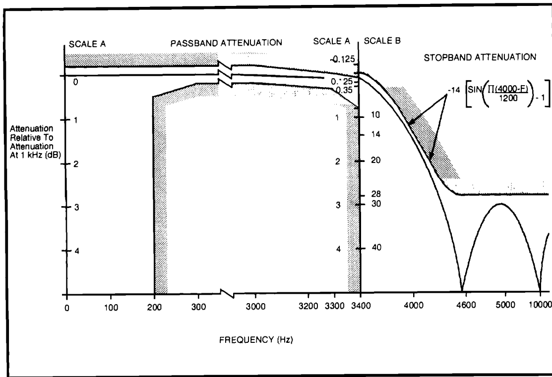
Figure 11 - Attenuation vs Frequency for Receive (D/A) Filter
