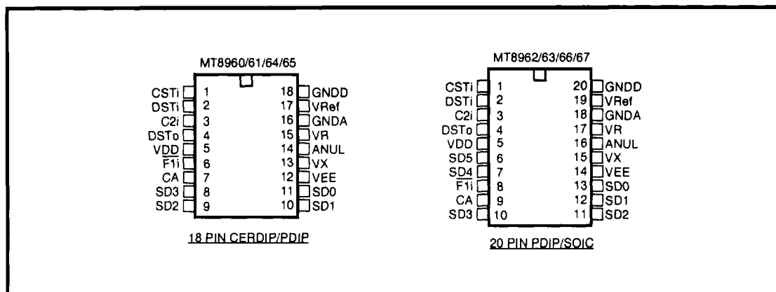
Figure 2 - Pin Connections
