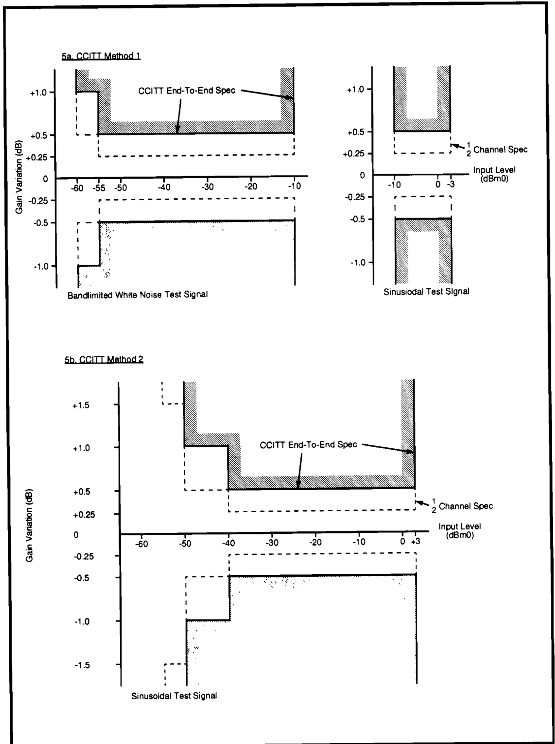
Figure 12 - Variation of Gain With Input Level
