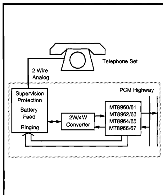
Figure 6 - Typical Line Termination
