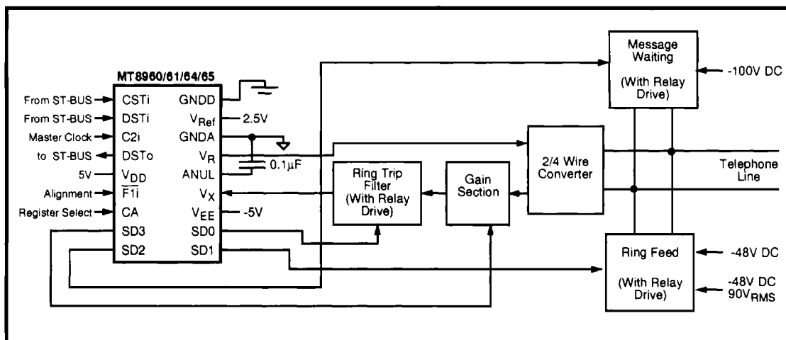
Figure 7 - Typical Use of the Special Drive Outputs
