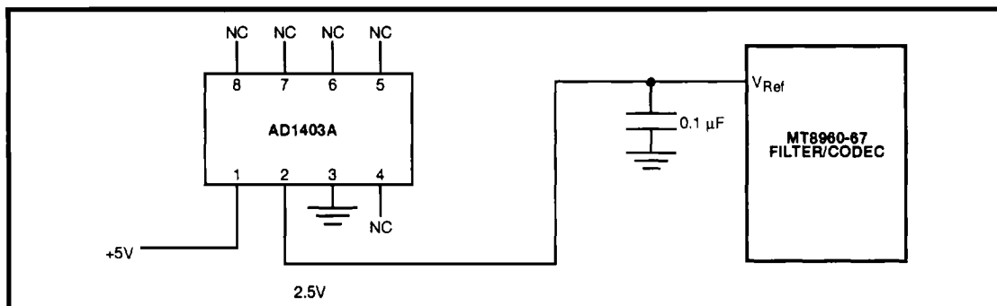
Figure 5 - Typical Voltage Reference Circuit
