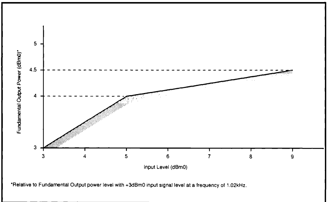
Figure 15 - Overload Distortion (End-to-End)
