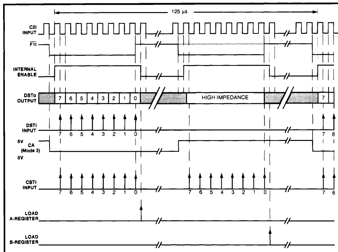
Figure 9a - Timing Diagram - 125µs Frame Period
