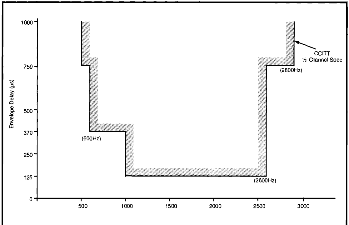
Figure 14 - Envelope Delay Variation Frequency
