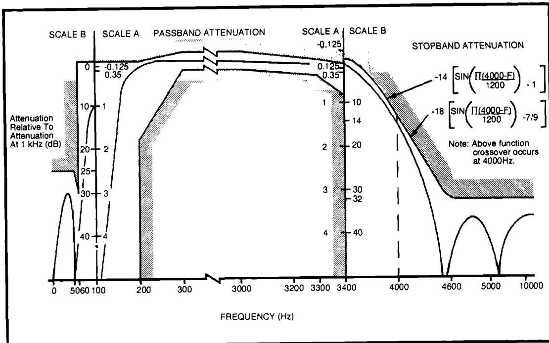
Figure 10 - Attenuation vs Frequency for Transmit (A/D) Filter
