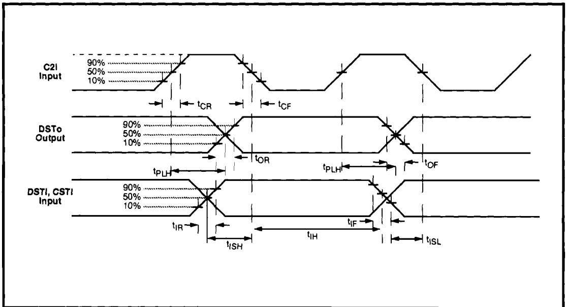
Figure 9c - Timing Diagram - Input/Output
