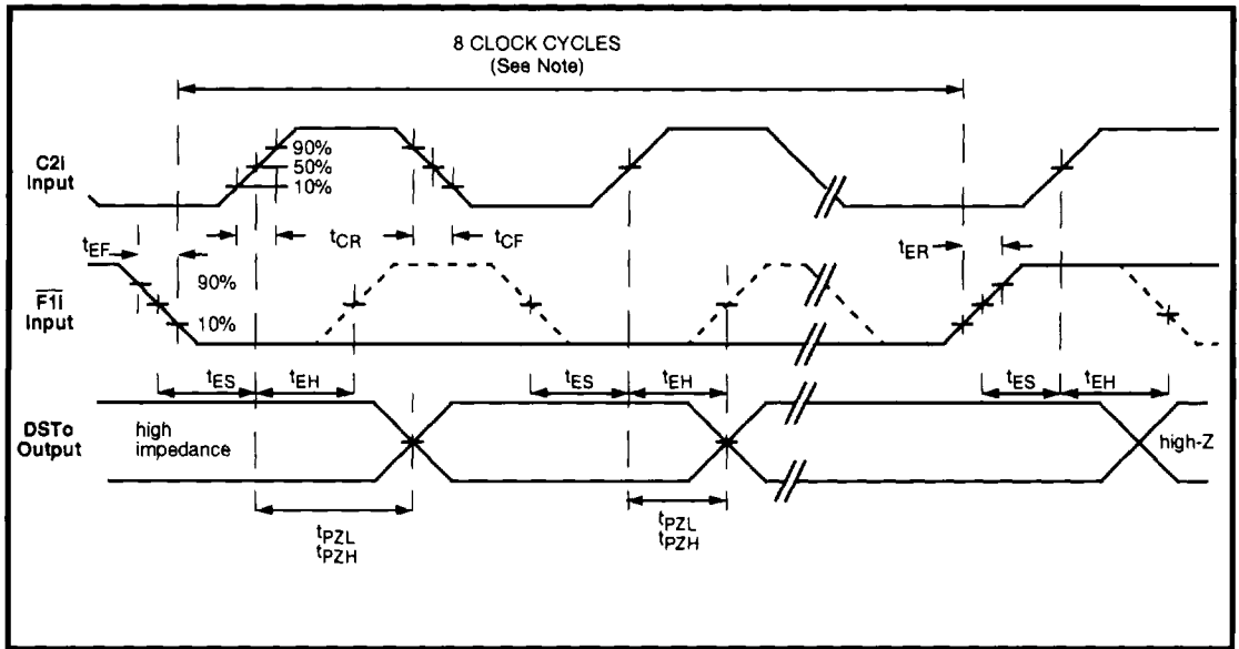
Figure 9b - Timing Diagram - Output Enable
