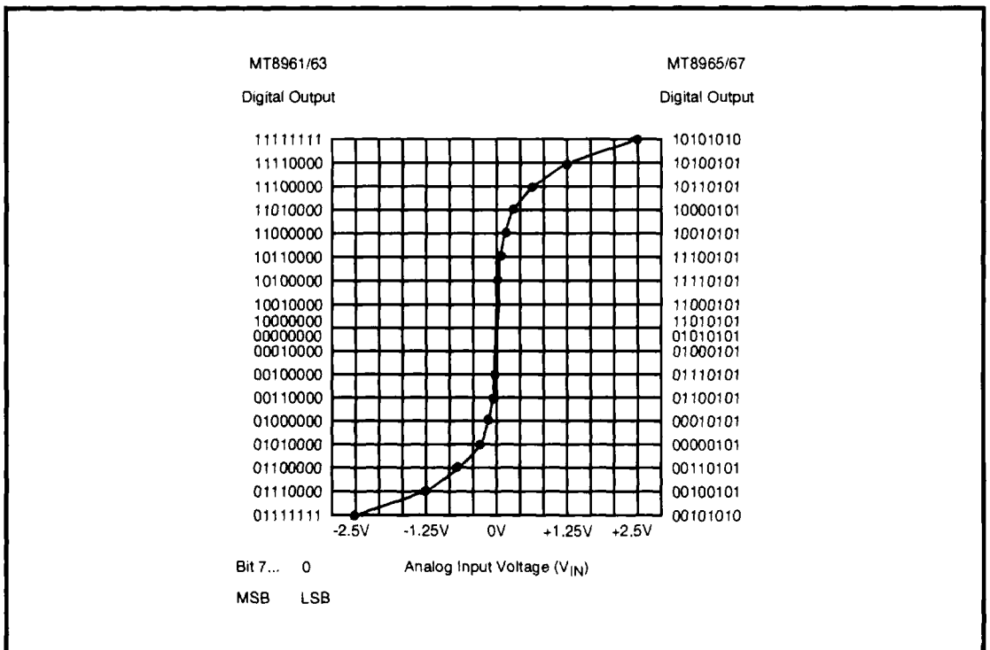
Figure 4 - A-Law Encoder Transfer Characteristic
