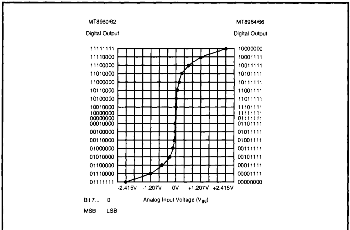
Figure 3 - \mu -Law Encoder Transfer Characteristic
