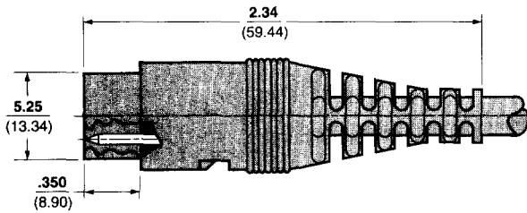
Male Assembly Part Number MDIN-5P-CABL
