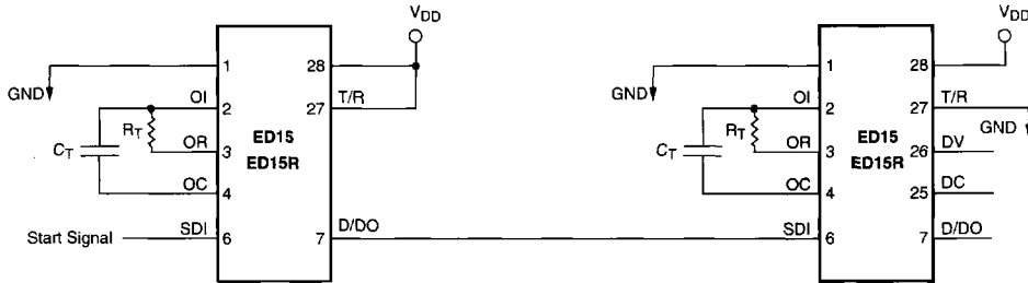
ED15 to ED15 and ED15R and ED15R
