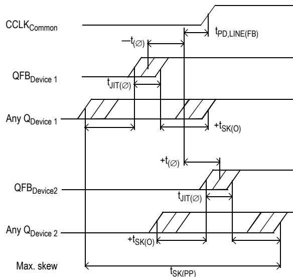
Figure 8. MPC93H51 maximum device-to-device skew
