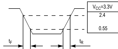
Figure 19. Output Transition Time Test Reference
