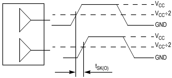
Figure 13. Output to output Skew t_{SK(O)}
