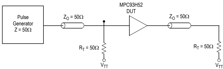
Figure 12. CLK MPC93H52 AC test reference for V_{CC} = 3.3V and V_{CC} = 2.5V
