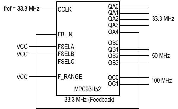
MPC93H52 configuration to multiply the reference frequency by 3, 3 2 and 1. PLL feedback of QA4 = 33.3 MHz.
