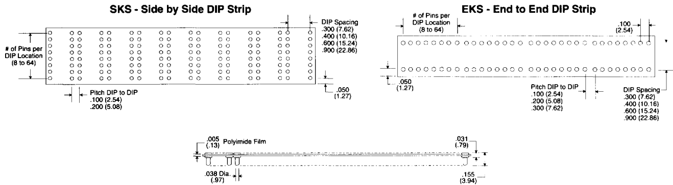
Side View - Terminal Type -85 Shown
