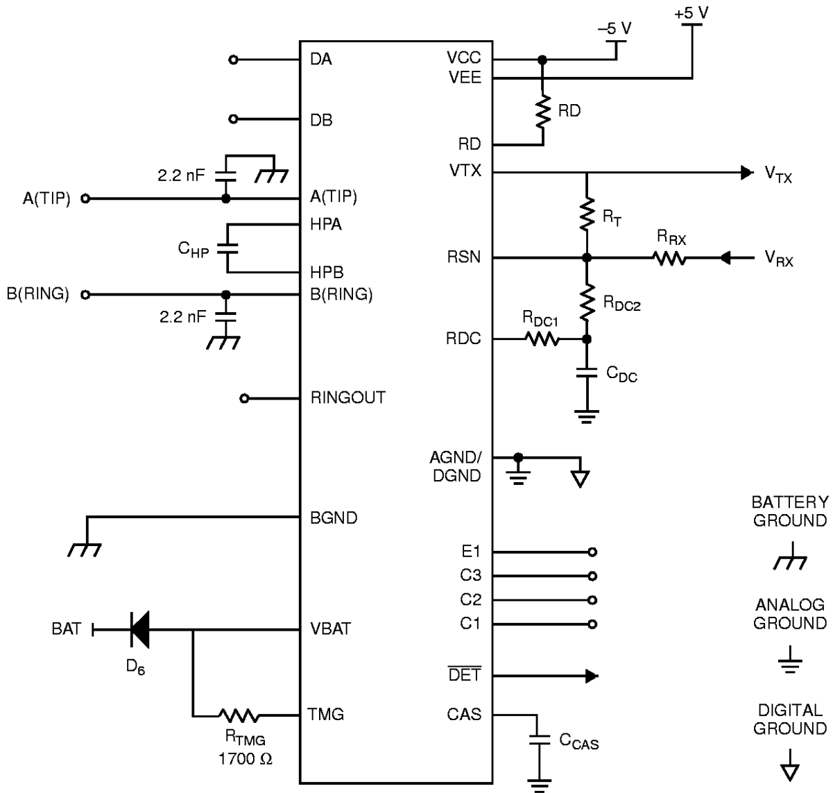
H. Am7945 Test Circuit
