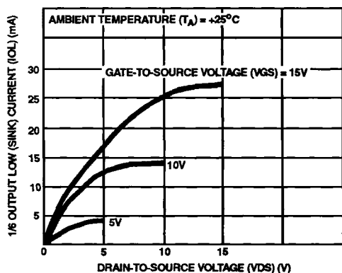
FIGURE 1. TYPICAL OUTPUT LOW (SINK) CURRENT CHARACTERISTICS
