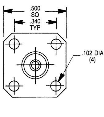
Mounting (a)
