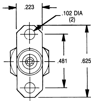
Mounting (c)
