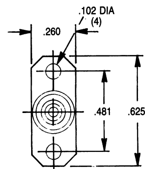
Mounting (b)
