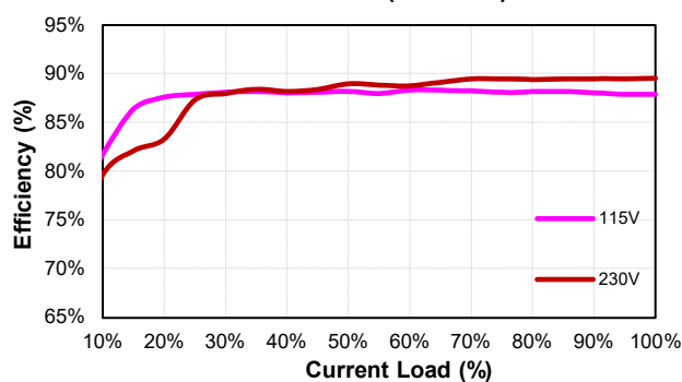
CFM81S150 (Eff Vs Io)
