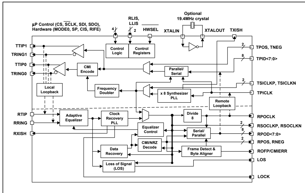
Figure 1. Intel® LXT6155 Block Diagram
