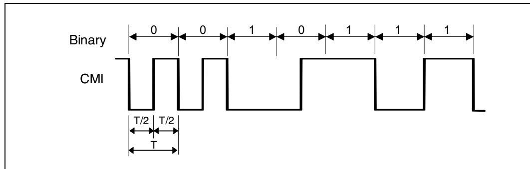
Figure 7. Example of CMI Encoded Binary Signal
