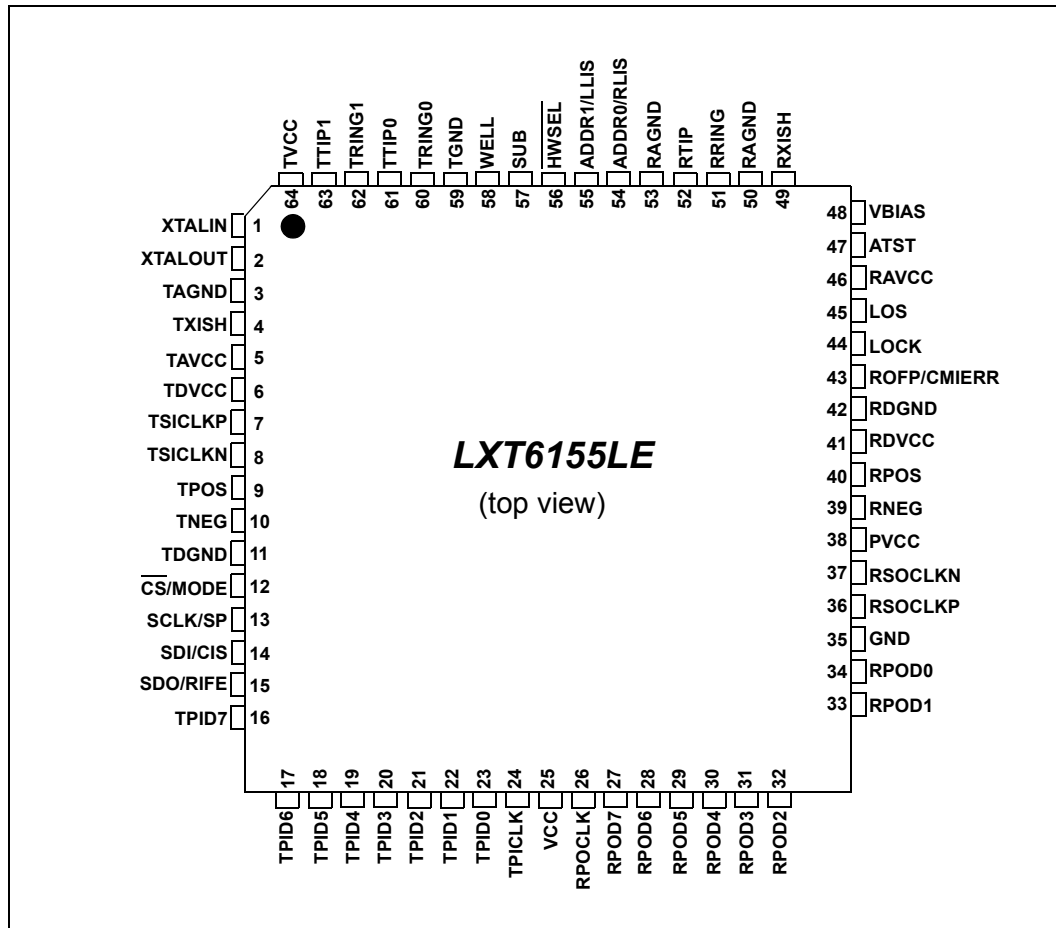
Figure 2. Intel® LXT6155 Pin Assignments
