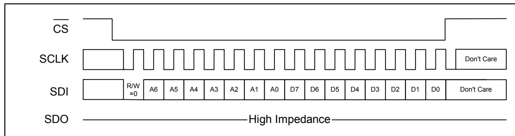
Figure 11. Serial Data Input Word Structure (Write Cycle: R/\overline{W} = Low)
