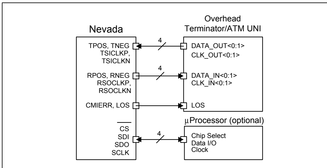
Figure 13. Parallel Interface
