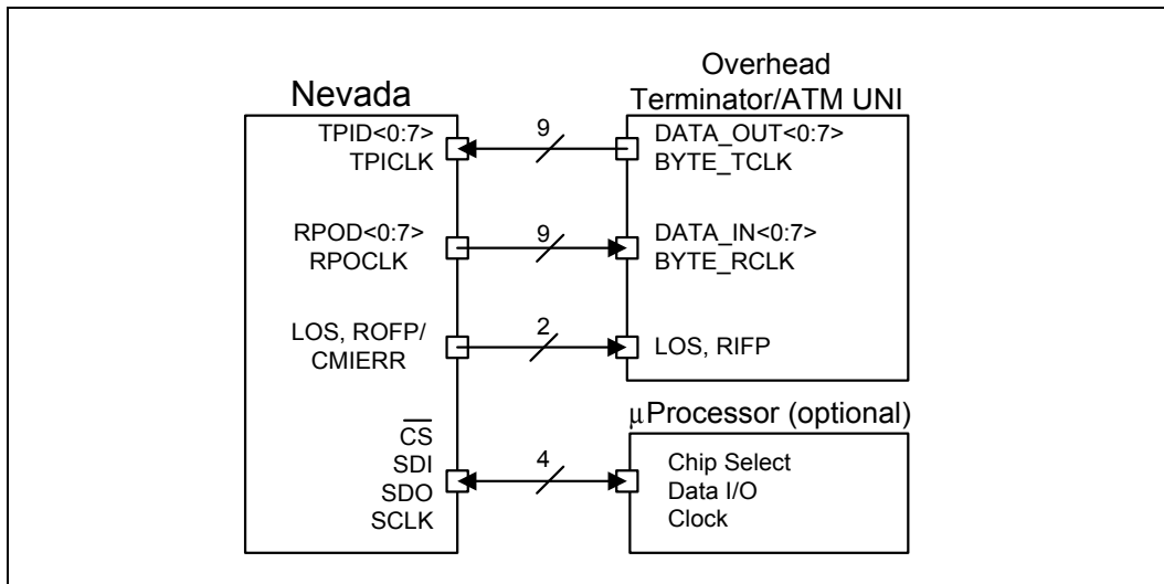
Figure 13. Parallel Interface
