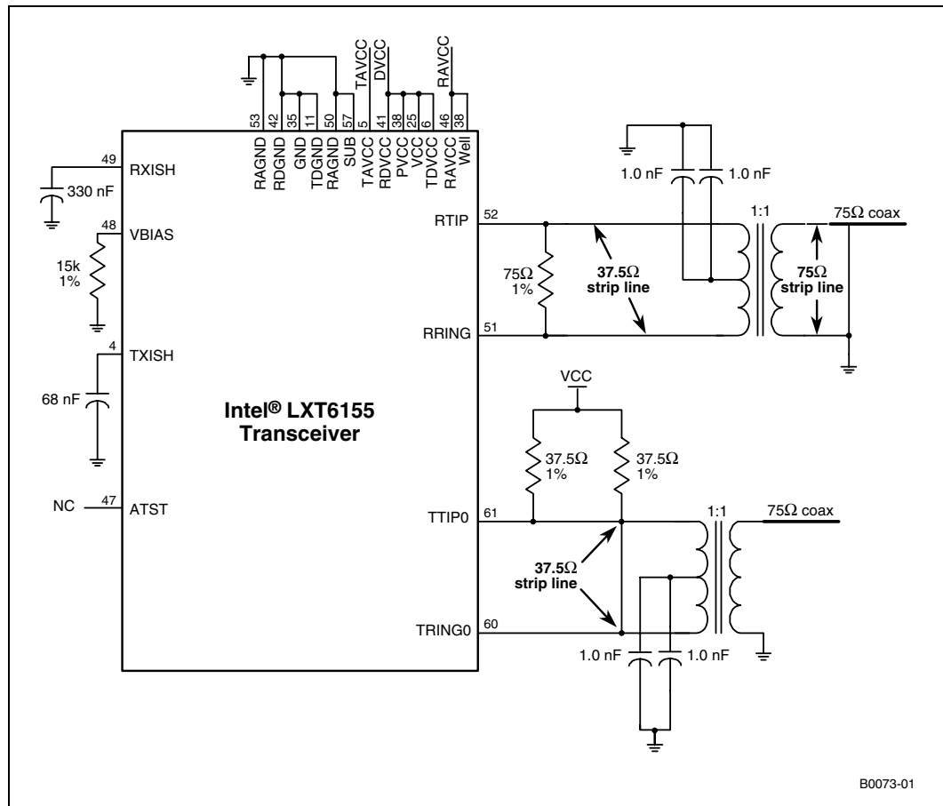
Figure 17. 75 Ω Coax Cable Interface
