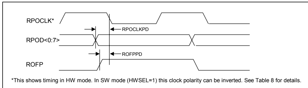
Figure 21. Receive Parallel Output Data Timing (See Table 31)
