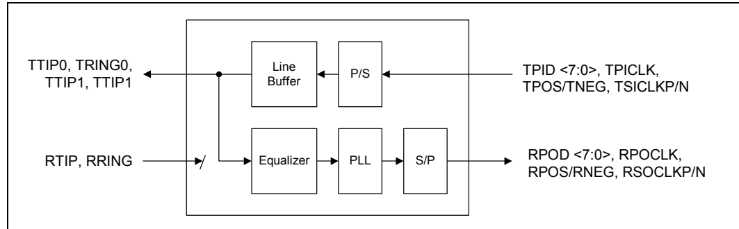
Figure 15. Remote Loopback
