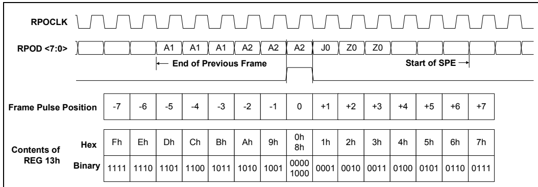
Figure 6. Receive Frame Synchronization and Frame Pulse Position
