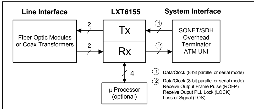
Figure 3. Intel® LXT6155 System Interface
