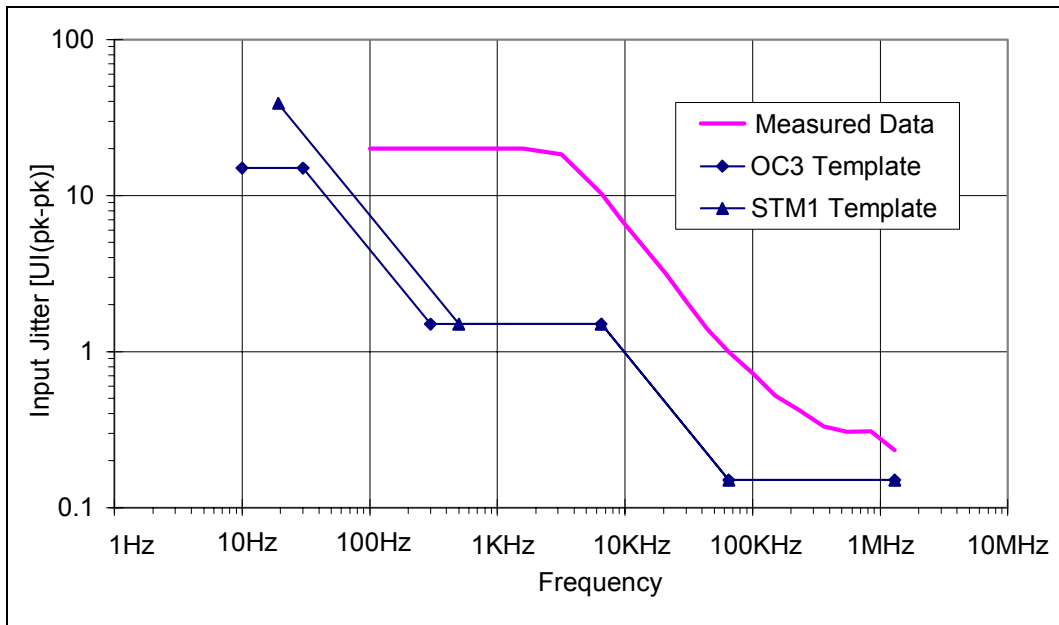
Figure 26. Jitter Tolerance
