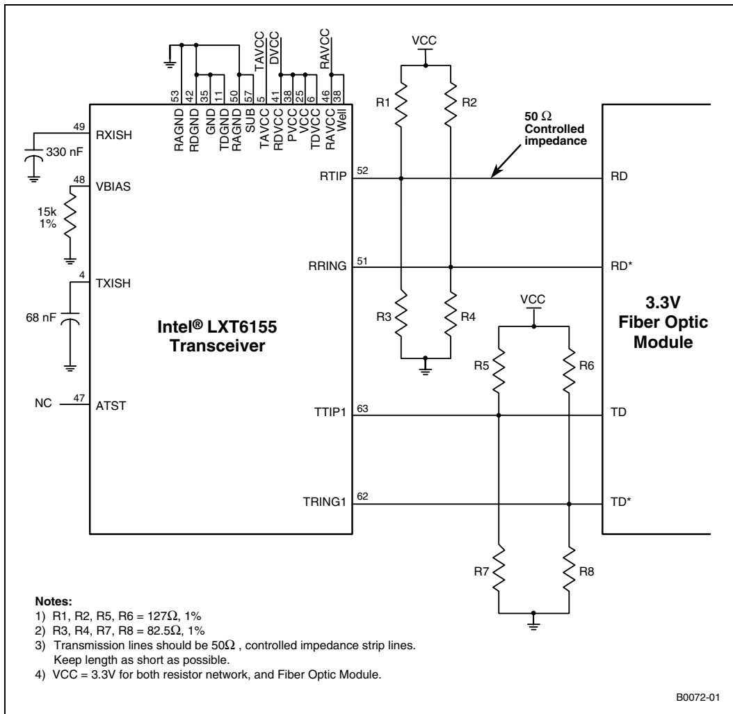
Figure 16. 3.3 V LVPECL to 3.3 V LVPECL Interface
