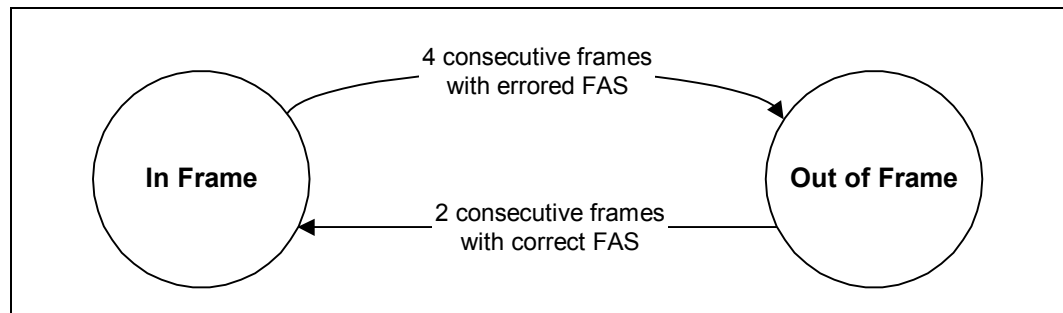
Figure 4. Framing State
