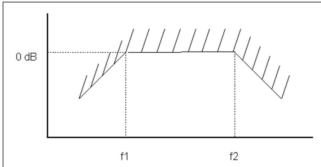
Figure 28. Typical Coax Jitter Transfer
