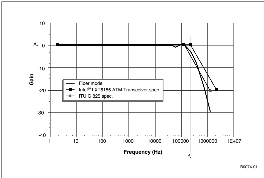
Figure 29. Typical Fiber Jitter Transfer
