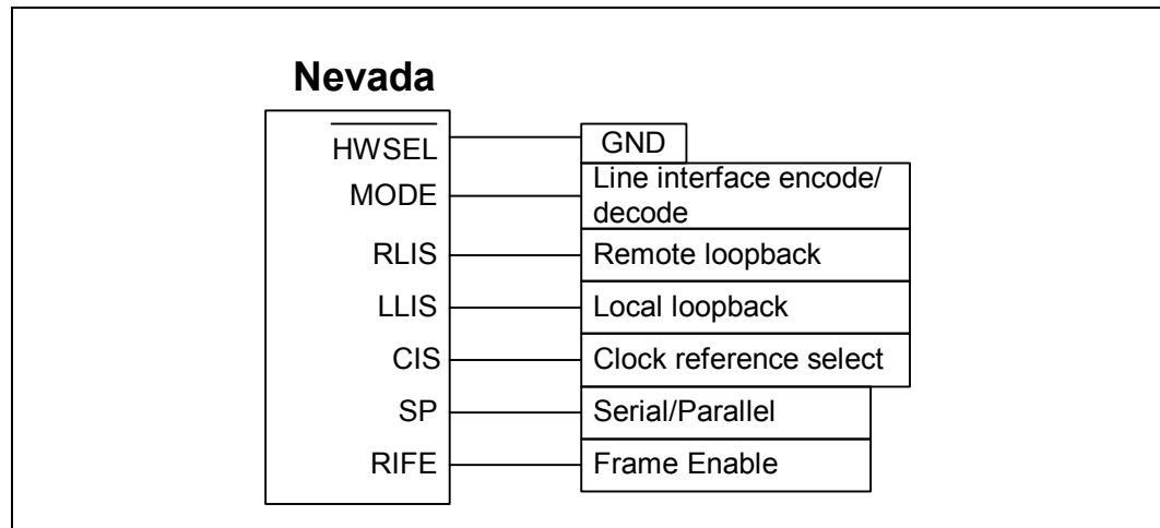
Figure 8. Hardware Mode
