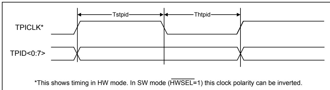
Figure 19. Transmit Serial Input Data Timing (See Table 29)
