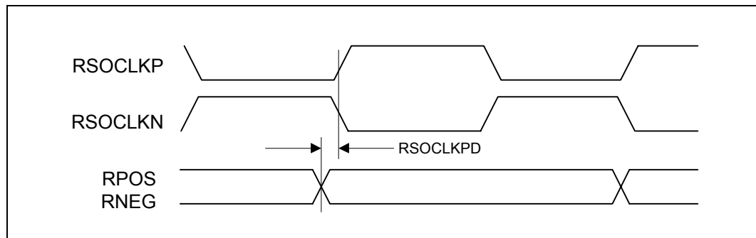
Figure 20. Receive Serial Output Data Timing (See Table 31)
