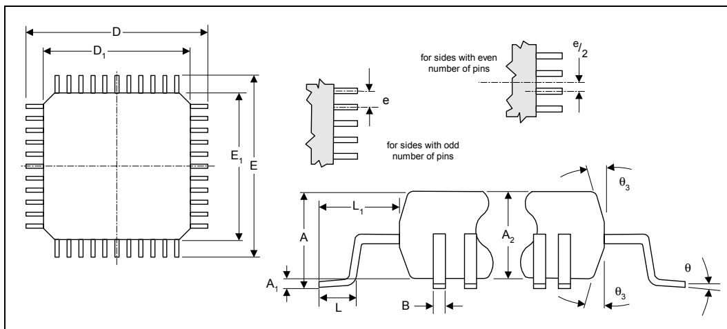
Figure 30. Intel® LXT6155LE Package Specification
