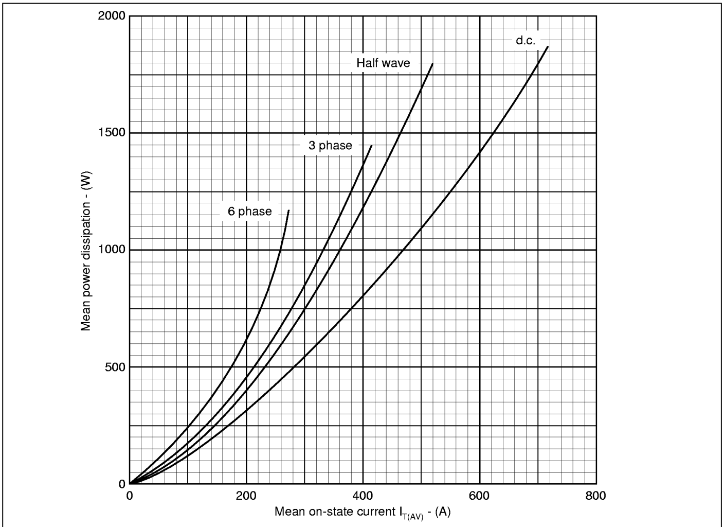
Fig.2 Dissipation curves
