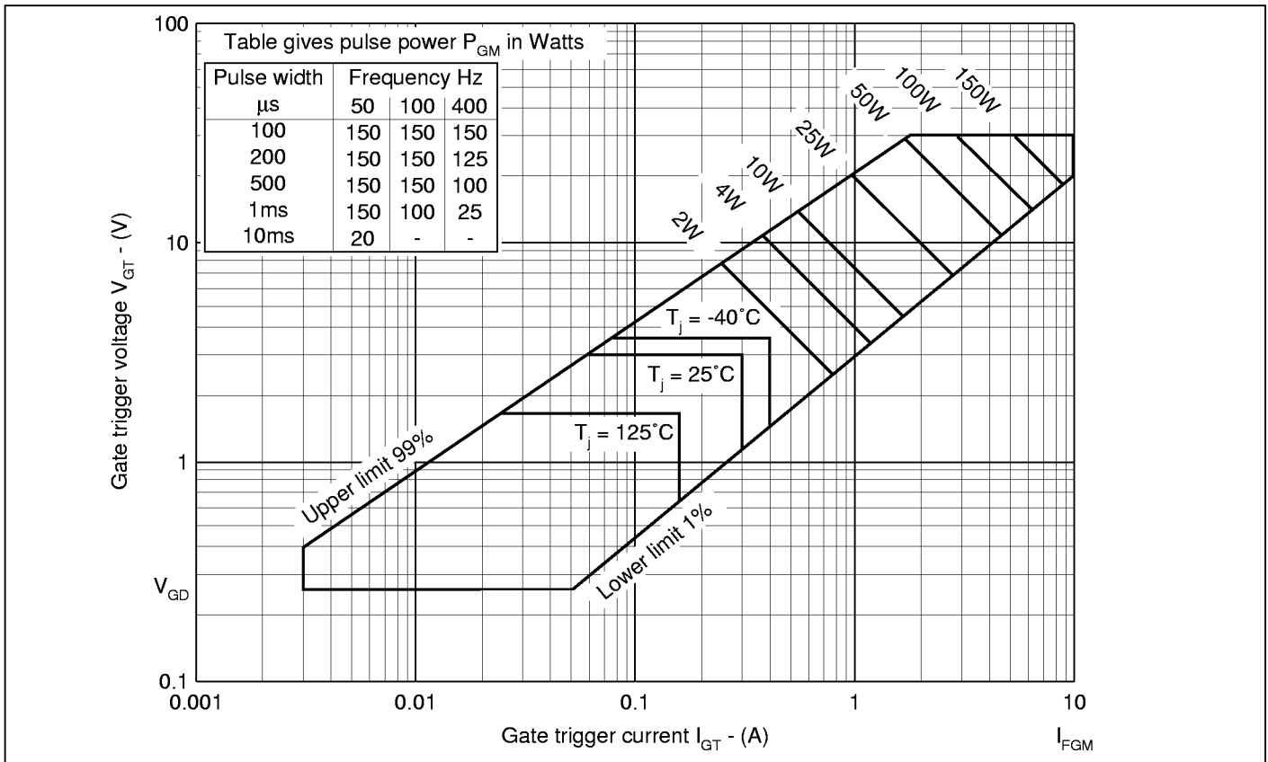
Fig.4 Gate characteristics
