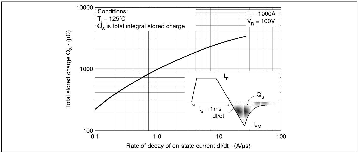
Fig.3 Stored charge
