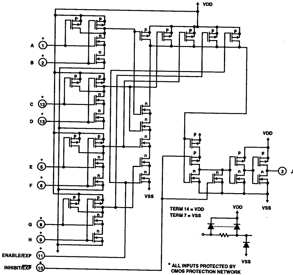
FIGURE 1. SCHEMATIC DIAGRAM
