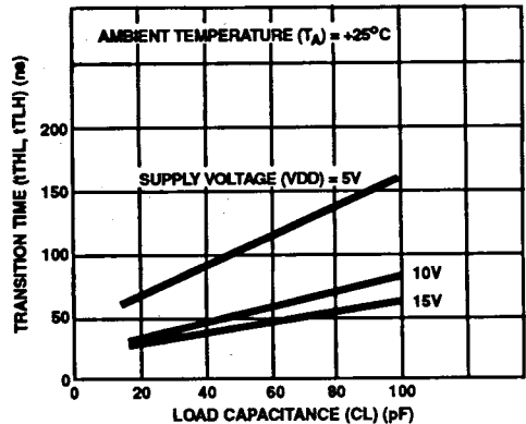
FIGURE 8. TYPICAL TRANSITION TIME vs LOAD CAPACITANCE
