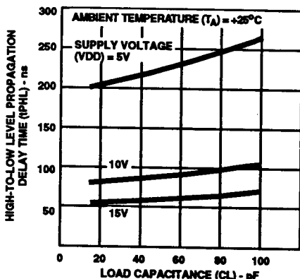
FIGURE 11. TYPICAL DATA OR ENABLE HIGH-TO-LOW LEVEL PROPAGATION DELAY TIME vs LOAD CAPACITANCE
