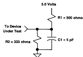
Fig. 3: Three-state Test Load
