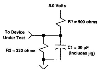
Fig. 2: TTL Switching Test Load
