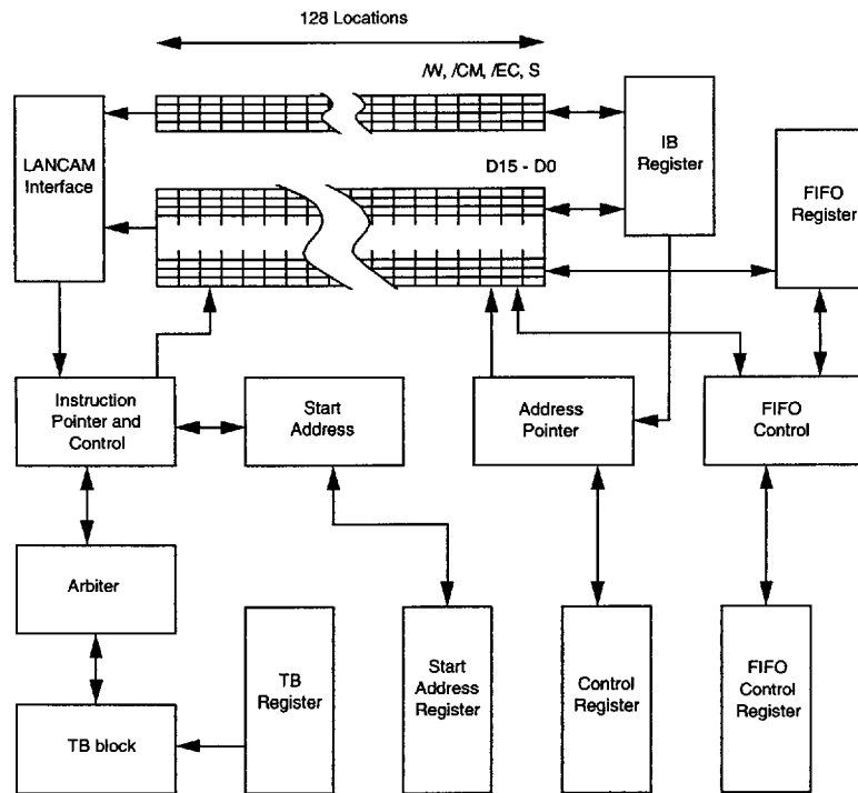
Figure 1: The Instruction Buffer
