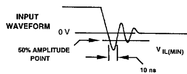
Fig. 5: Input Signal Waveform
