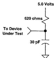
Fig. 4: Open-drain Test Load
