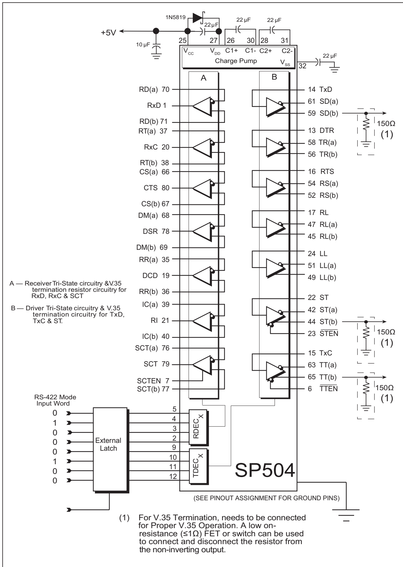
Figure 18. Typical Operation Circuit
