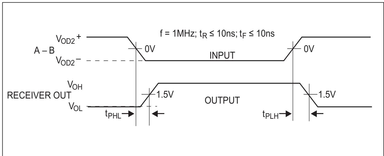
Figure 7. Receiver Propagation Delays
