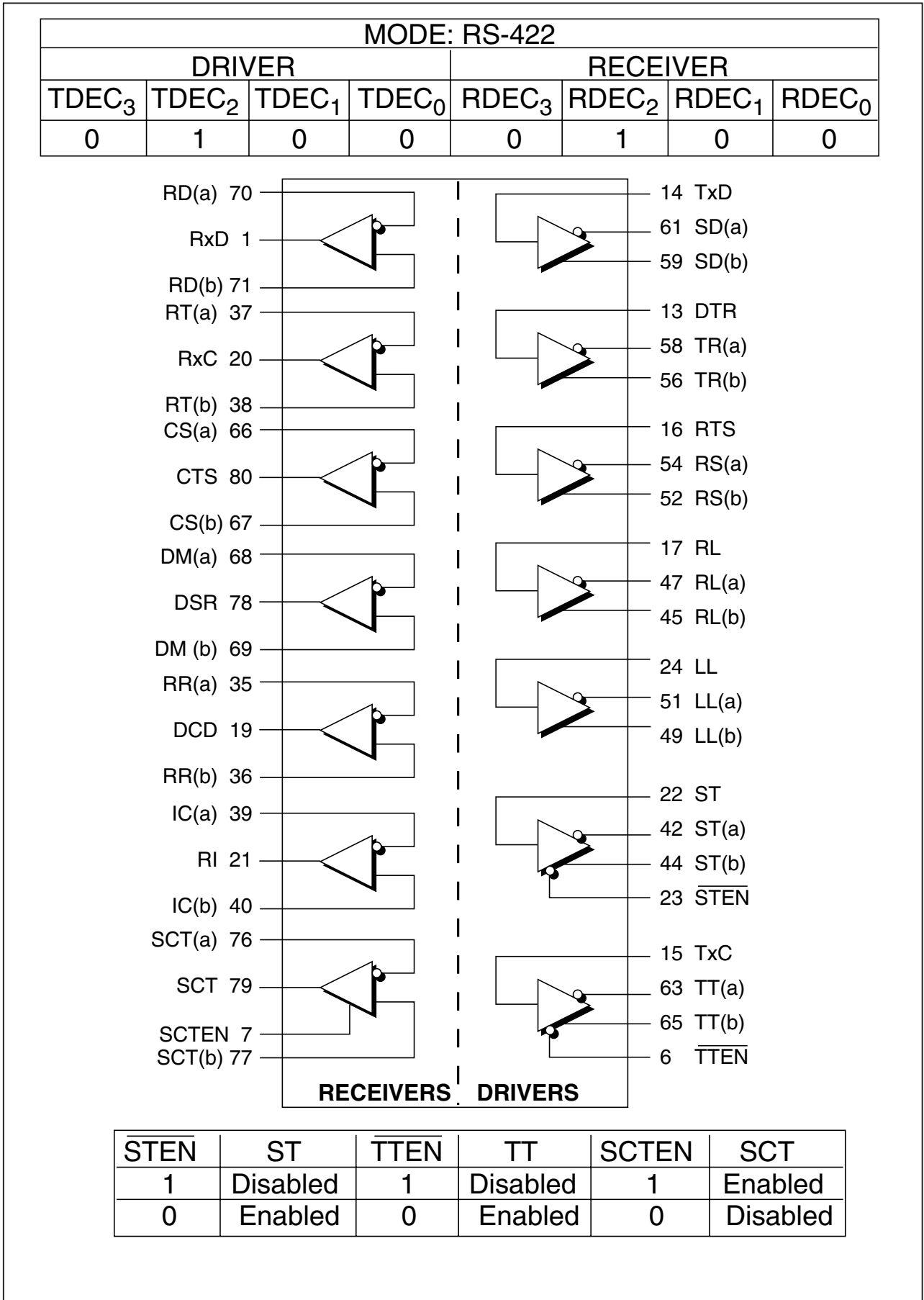
Figure 21. Mode Diagram — RS-422
