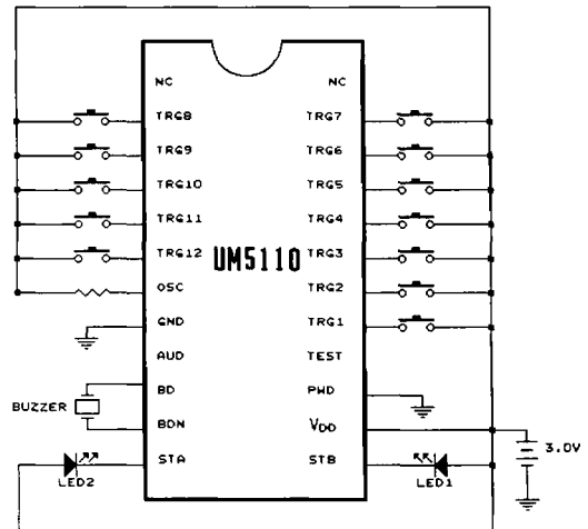
(b) Buzzer Output
