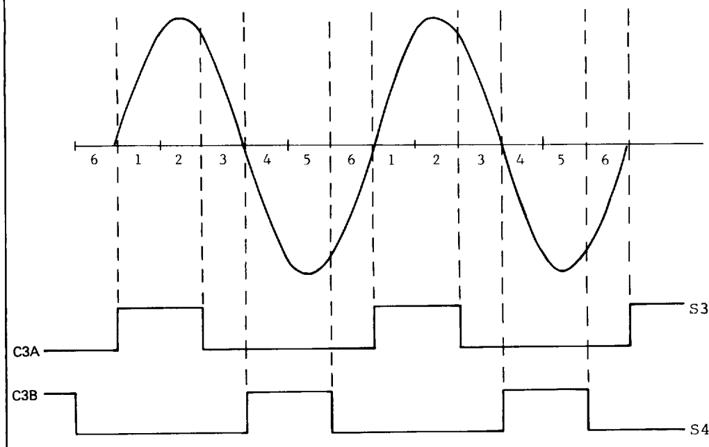
WORD SAMPLING WAVEFORMS FIG. 3
