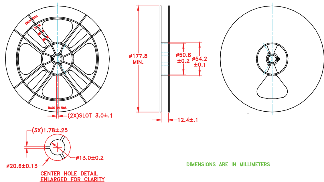
Figure 14: Carrier Tape
