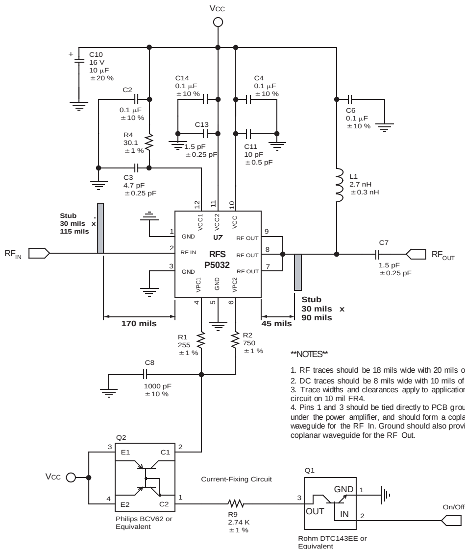
Figure 7: Application Circuit
