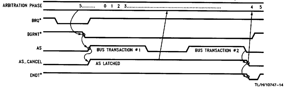
D. Multiple Accesses, AS_CANCEL Timing Diagram (AS is tied directly to the AS_CANCEL input of the Arbitration Controller. The Master must guarantee that the second transfer, or ENDT*, will come within 1 μs of the falling edge of the initial transfer AS signal).
