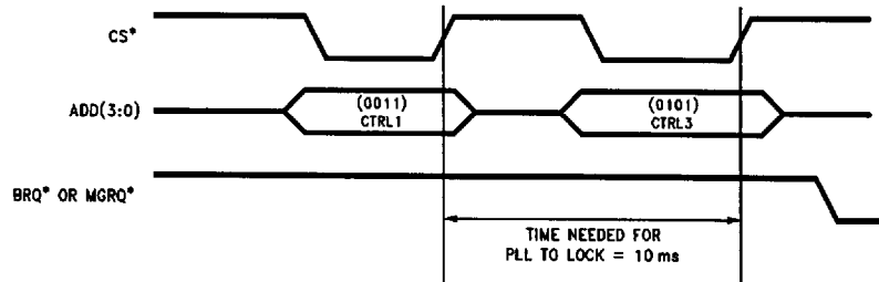
FIGURE 10c. PLL Lock Period
