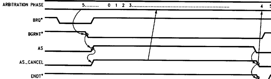
FIGURE 6b. Timing of the AS_CANCEL Signal
