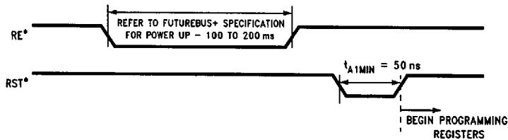
FIGURE 10a. Programming Registers: After Power-Up
