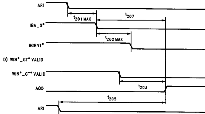
C. IBA Mode Selected-Winner of Competition
