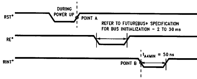
FIGURE 10b. Programming Registers: During Bus Initialization
