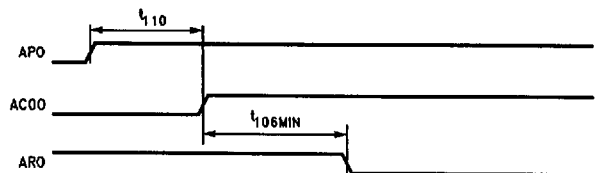
E. Asserting AC00 - Slow Mode (F_S*) Is Selected
