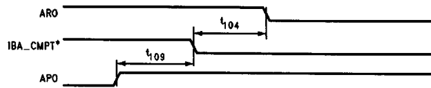
C. IBA Mode Selected
