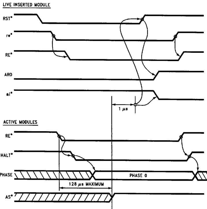
FIGURE 11. Live Insertion
