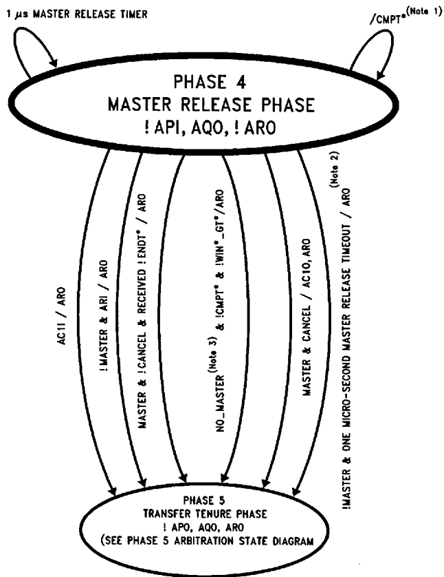
FIGURE 7e. Phase 4 Arbitration State Diagram
