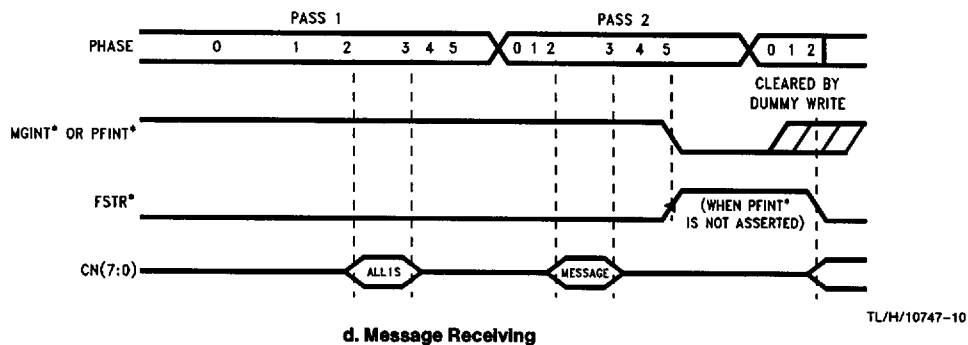
d. Message Receiving
