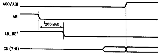
B. Register Access CN Port-Input
