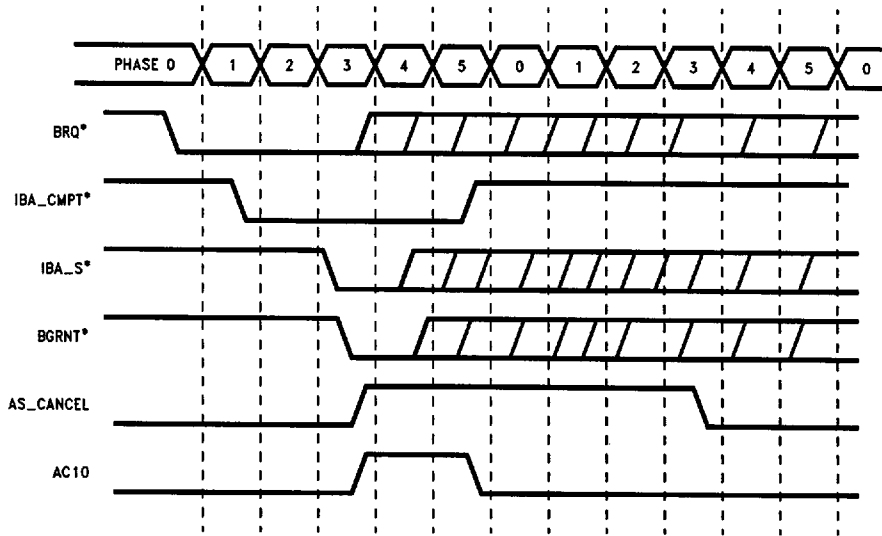
FIGURE 12b. IBA—Unrestricted Two Pass
