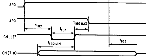
B) REGISTER ACCESS CN PORT - OUTPUT
