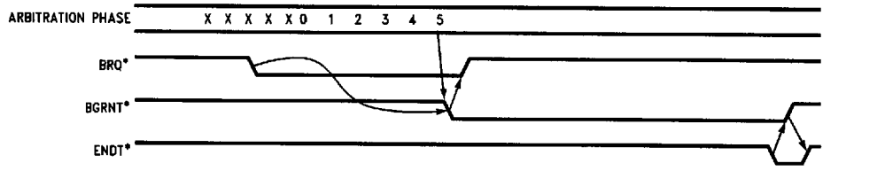
a. Normal Bus Request Timing
