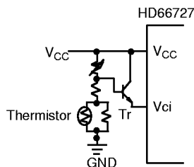
Figure 35 Temperature Compensation Circuit Example
