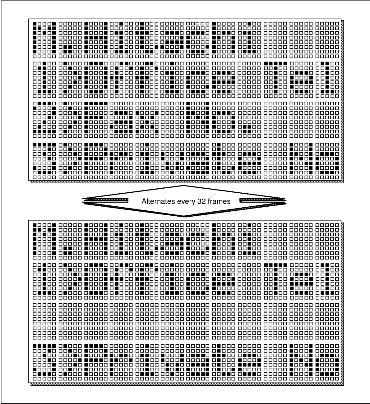
Figure 45 Example of Blink Cursor (LC = 1; B = 1)
