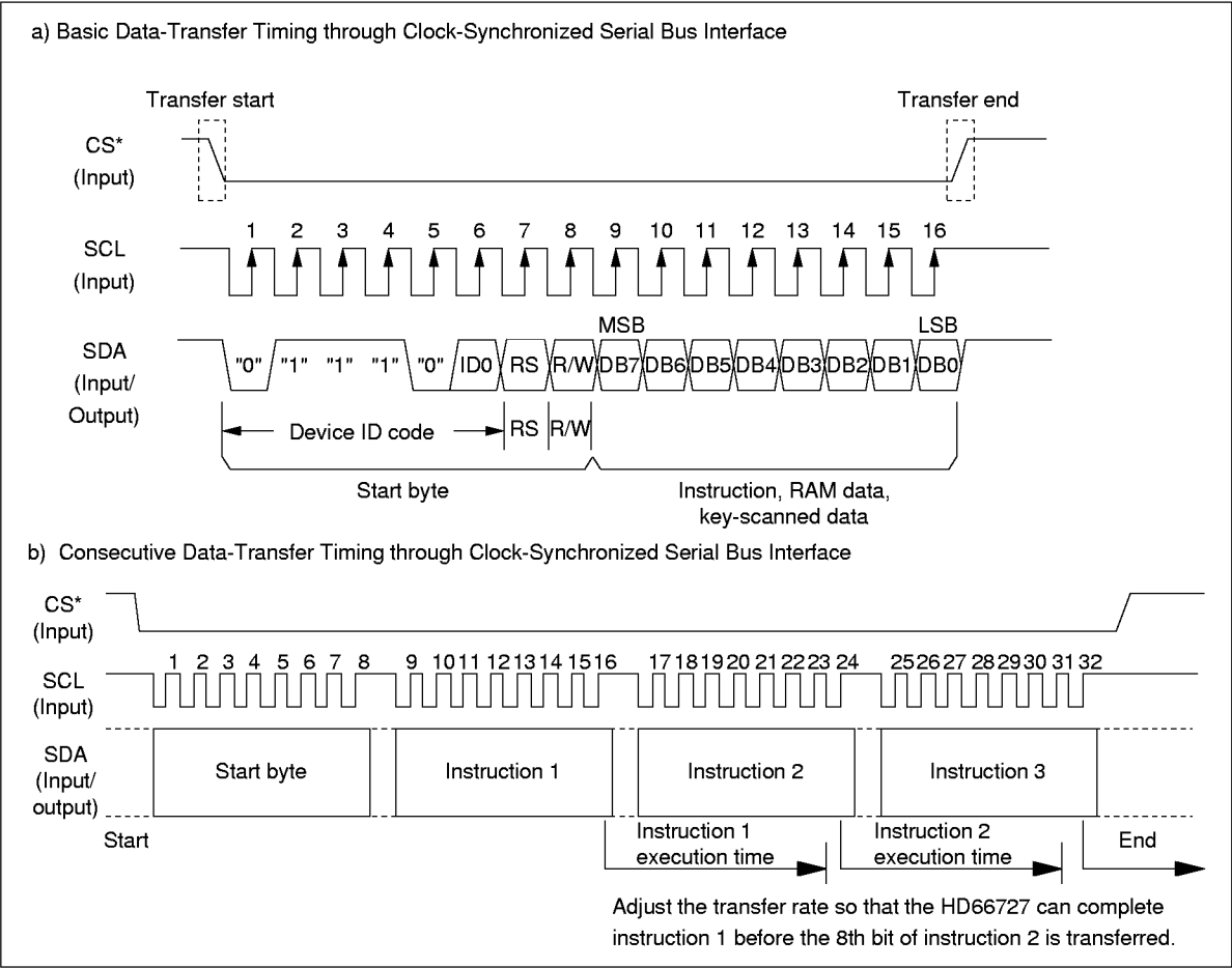
Figure 24 Clock-Synchronized Serial Interface Timing Sequence
