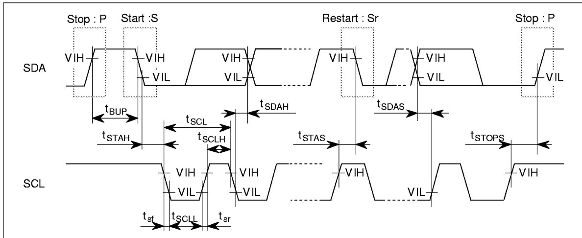
Figure 59 I 2 C Bus Interface Timing
