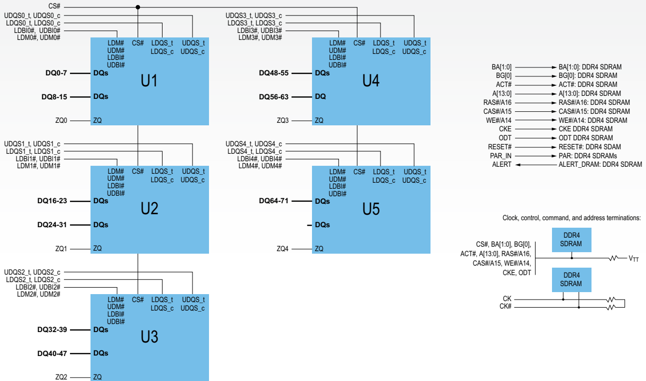
Figure 2 - Block Diagram for the x72 Device
