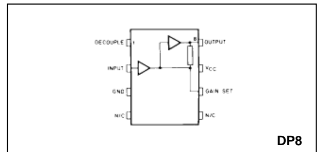
Fig.2 Pin connections (view as above) SL561C
