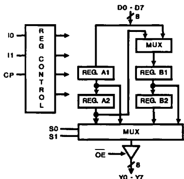
FUNCTIONAL DIAGRAM
