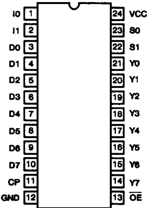
TERMINAL ASSIGNMENT
