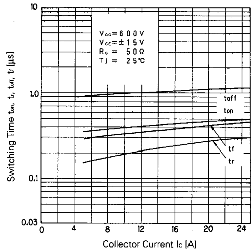
Switching Time
