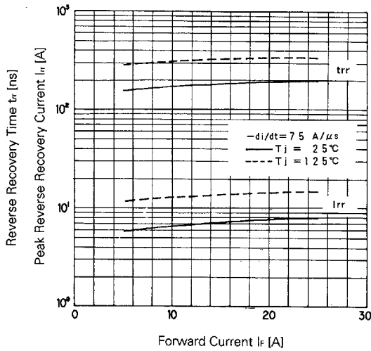
T_{rr}, I_{rr}-I_f
