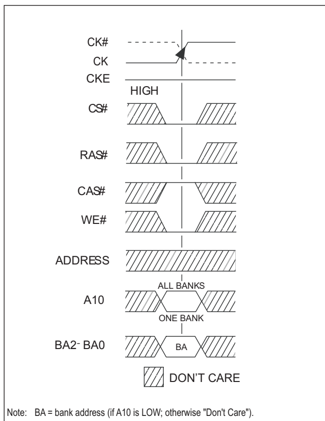
FIGURE 13 – PRECHARGE COMMAND
