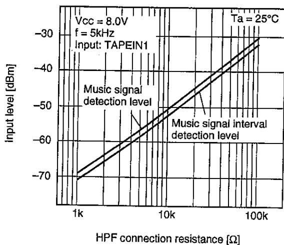
HPF connection resistance in MS block vs. Music signal and signal interval detection level characteristics
