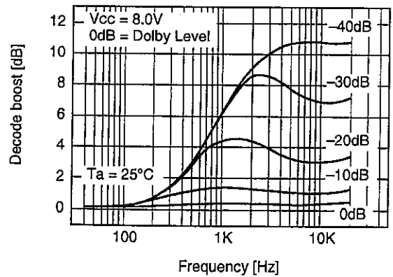
B type decode boost characteristics
