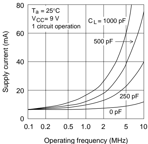
Supply current vs. operating frequency (HD29026A)
