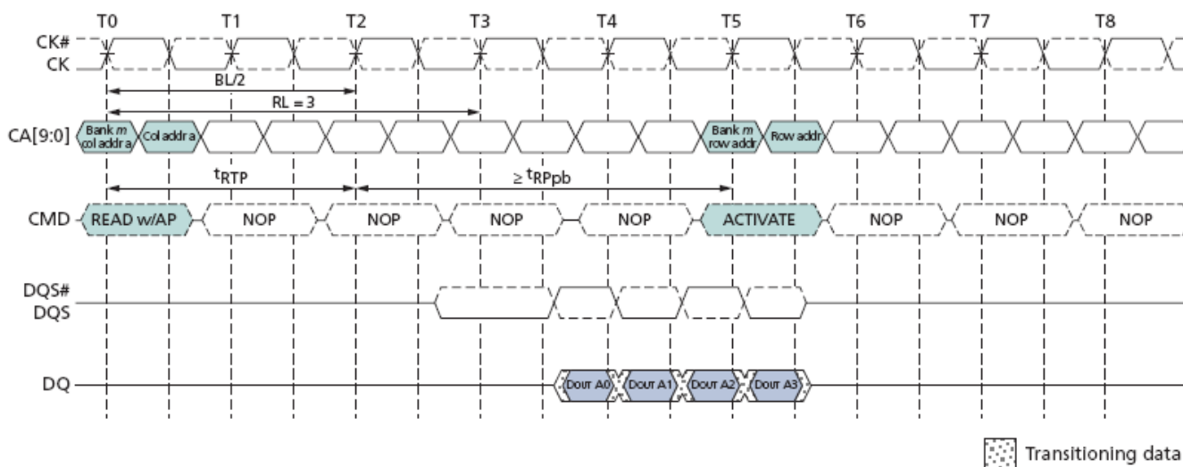
Burst Read with Auto-Precharge: RL=3 , BL=4 , RU(t_{RTP(min)}/t_{CK})=2
