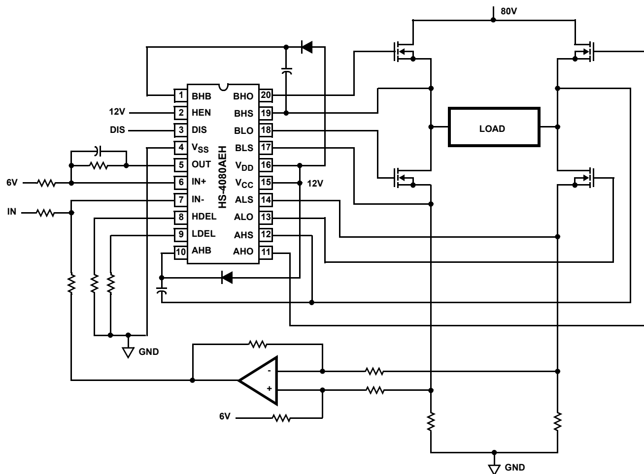
FIGURE 2. TYPICAL APPLICATION
