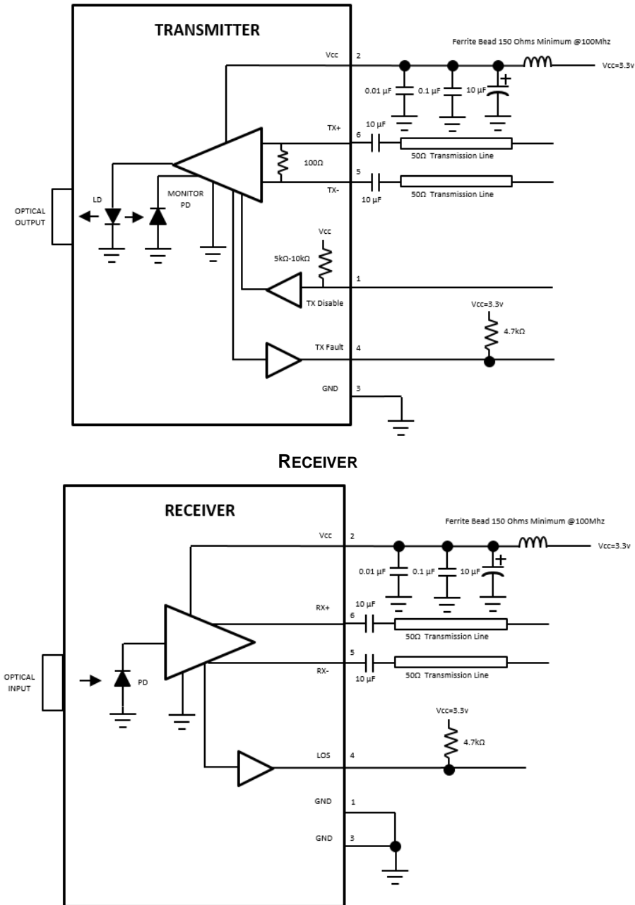
FIGURE 3 RECOMMENDED BOARD HOST BOARD SCHEMATIC TRANSMITTER
