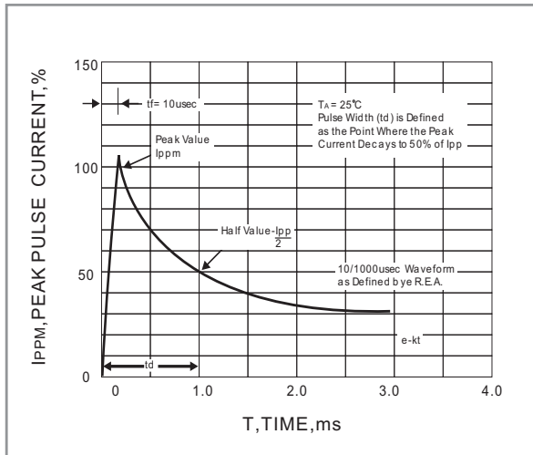
Fig.3 PULSE WAVEFORM
