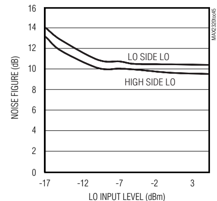
CELLULAR-BAND FM MIXER NOISE FIGURE vs. LO INPUT LEVEL
