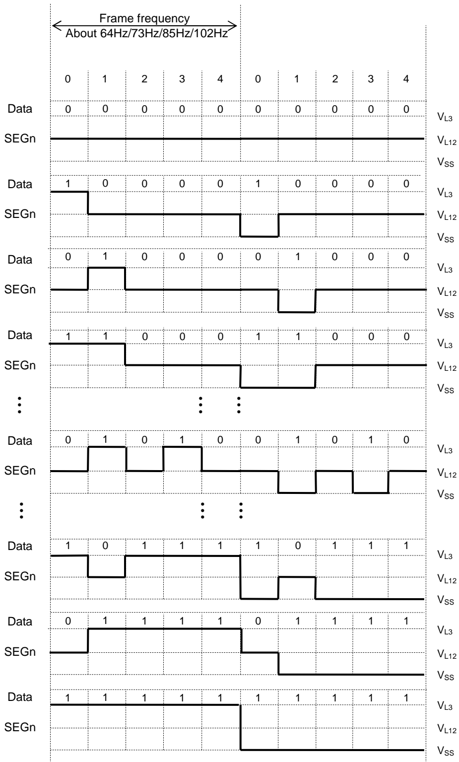
Figure 22-12 Segment Output Waveform at 1/5 Duty (5 Commons) and 1/2 Bias
