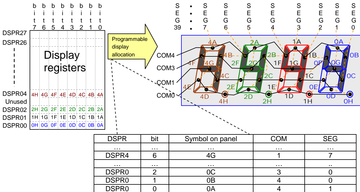
Figure 22-3 An example of correlation between display registers and segment type LCD
