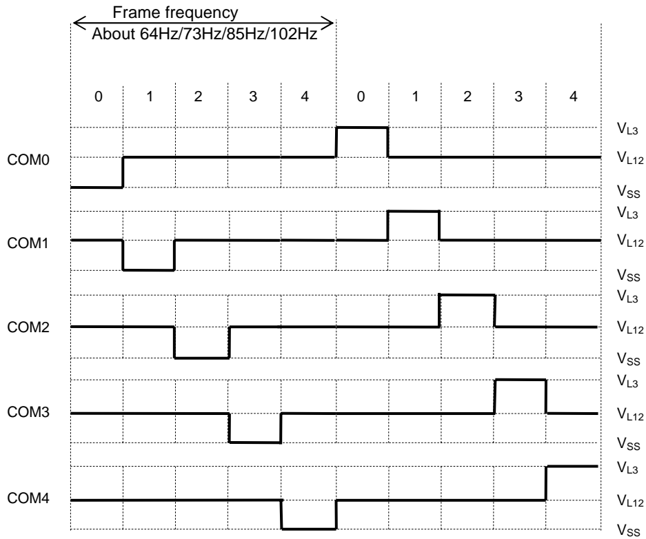
Figure 22-10 Common Output Waveform at 1/5 Duty (5 Commons) and 1/2 Bias
