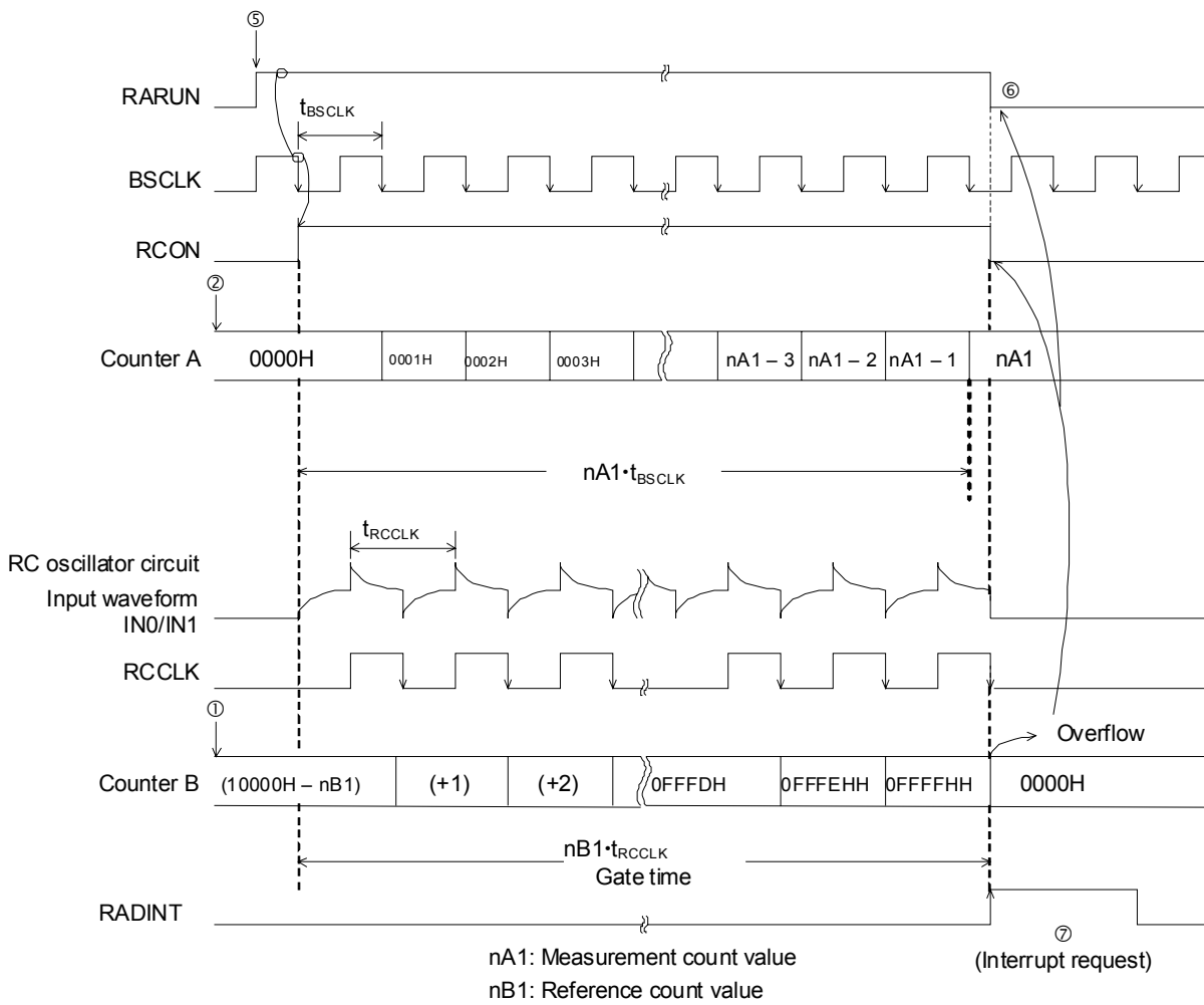
Figure 21-7 Operation Timing in Counter B Reference Mode
