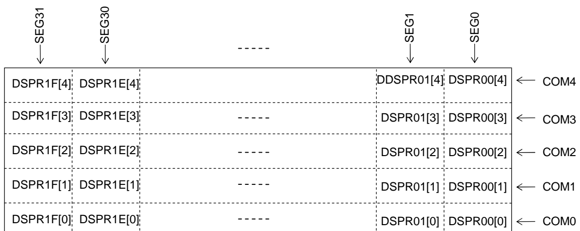
Figure 22-7 Segment Map Configuration Diagram
