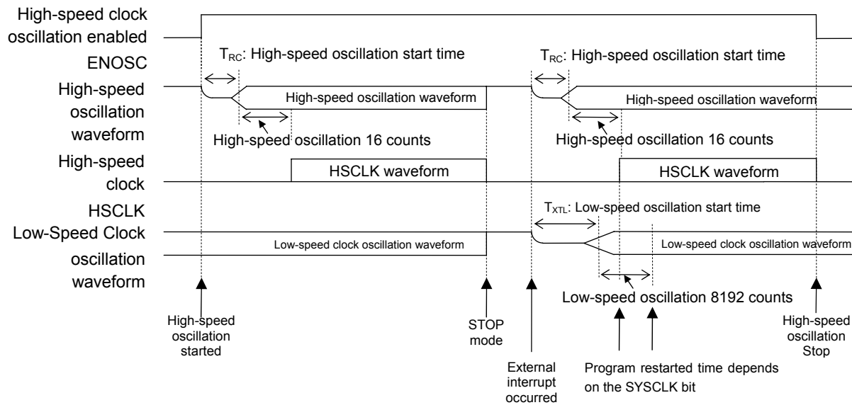
Figure 6-5 Operation of High-Speed Clock Generation Circuit
