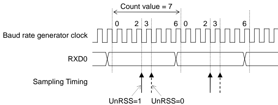
(1) When the baud rate generator count value is "7" (odd)
