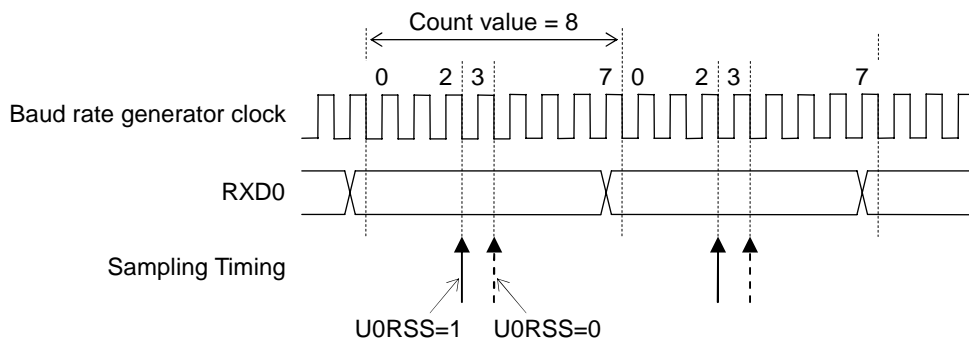
(2) When the baud rate generator count value is "8" (even)
