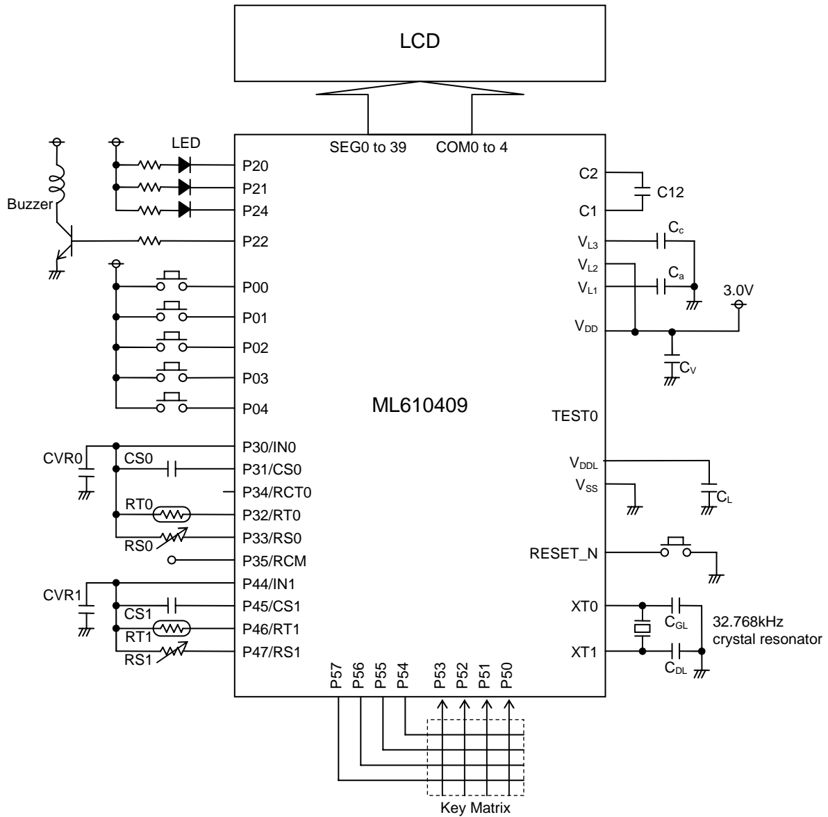
Figure D-1 ML610409 Application Circuit Diagram
