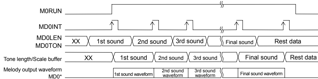
Figure 20-2 Operation Waveform of Melody Driver
