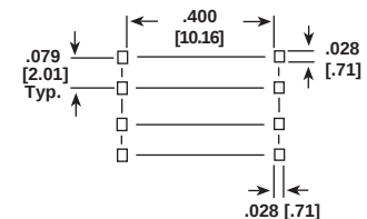
Footprint Diagram
