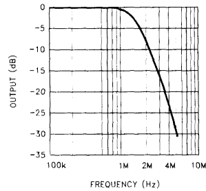
Input Signal = 300mV p-p EL4581C Filter Characteristic Constant Delay 240 ns
