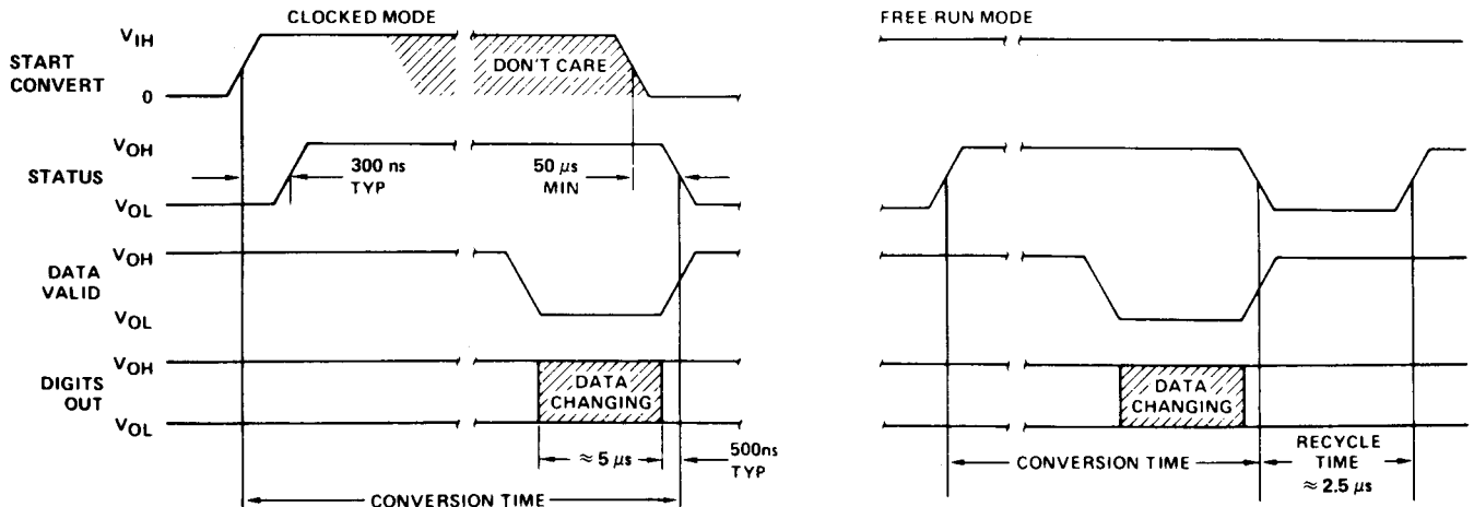
Figure 3. Timing Diagrams (Rise, fall times = 200 ns typ., C_L = 50 pF)
