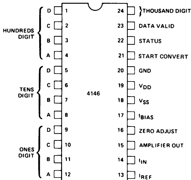
Figure 1. 4146 Pin Out
