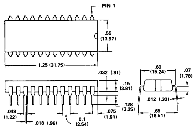
4146 24-Pin Plastic DIP
