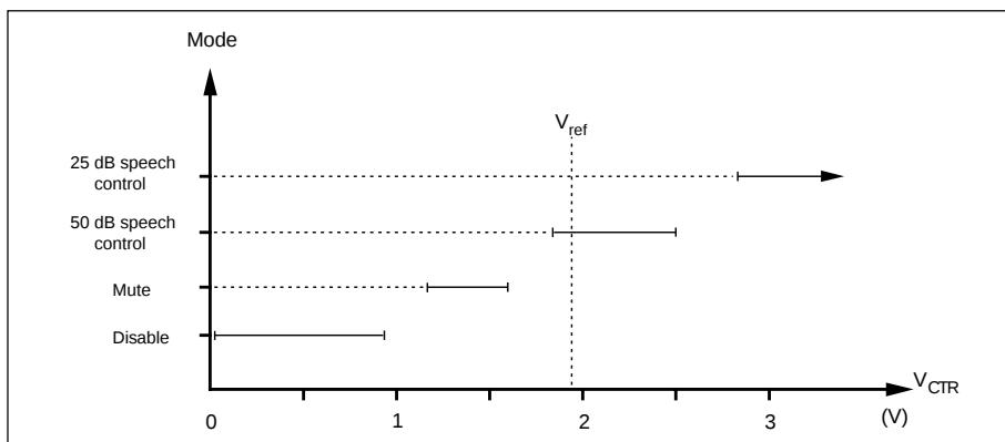
Figure 15. Control modes as function of voltage applied to gain dynamics control input CTR I_O=1mA
