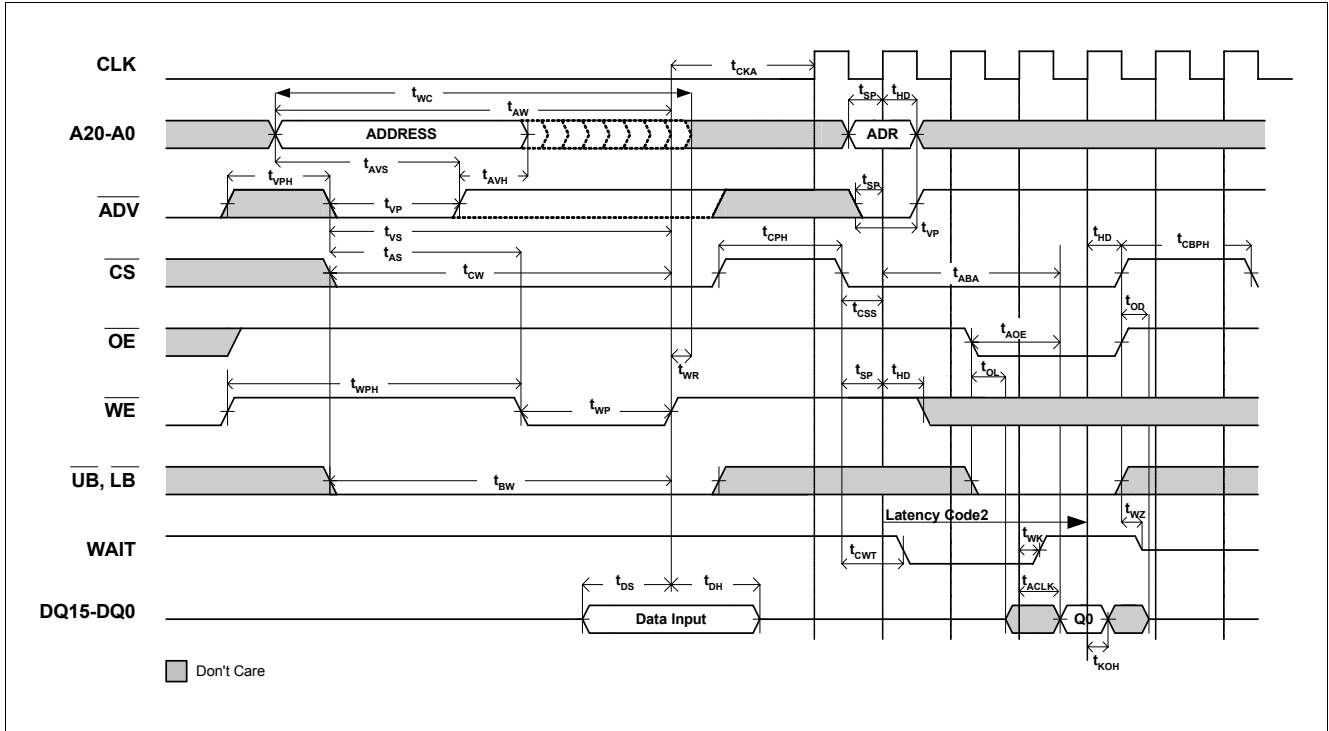
Figure 21 Asynchronous Write with Address Latch ( \overline{\text{ADV}} ) Control (followed by single-burst read)
