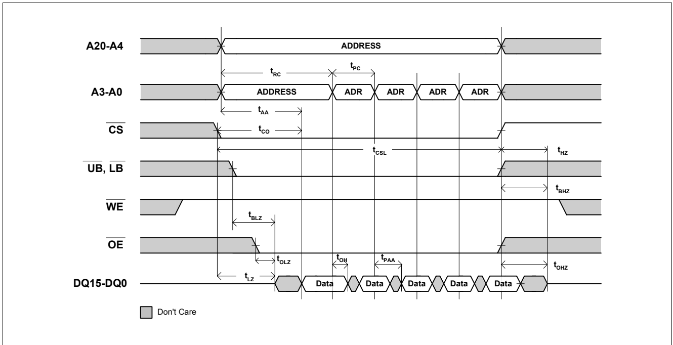
Figure 14 Asynchronous Page Read Mode ( CRE = V_{IL}, \overline{ADV} = V_{IL} )
