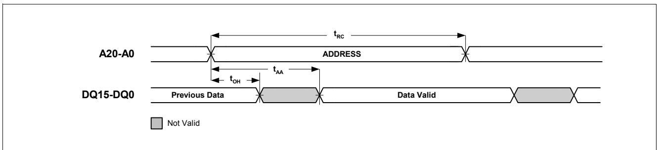
Figure 12 Asynchronous Read - Address Controlled ( \overline{CS} = \overline{OE} = V_{IL} , \overline{WE} = V_{IH} , \overline{UB} and/or \overline{LB} = V_{IL} , CRE = V_{IL} , \overline{ADV} = V_{IL} )
