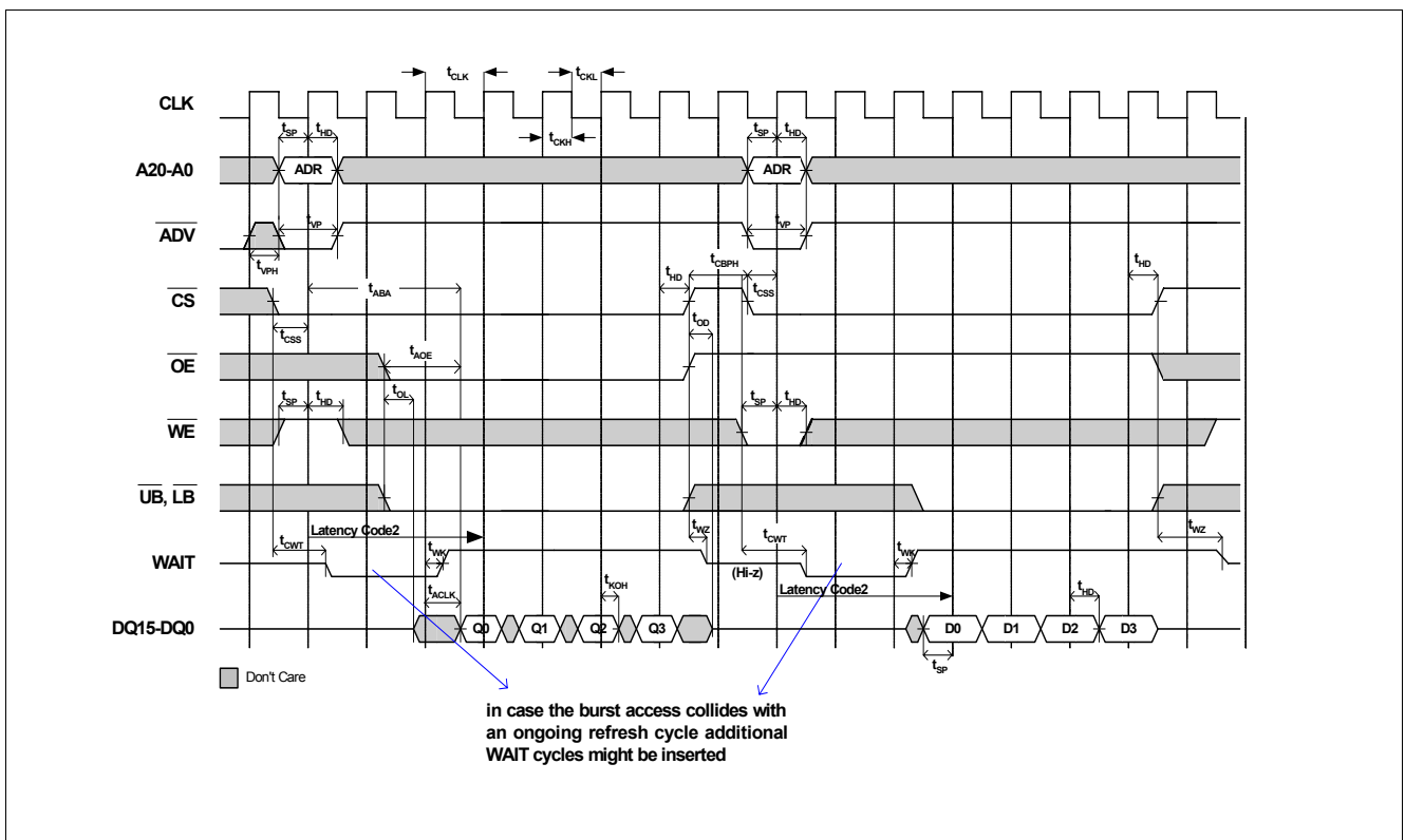
Figure 27 Synchronous Read Burst Followed by Synchronous Write Burst
