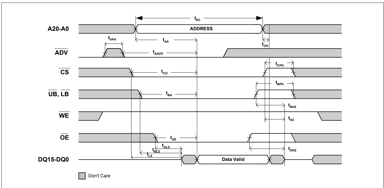
Figure 13 Asynchronous Read ( \overline{WE} = V_{IH} , CRE = V_{IL} )
