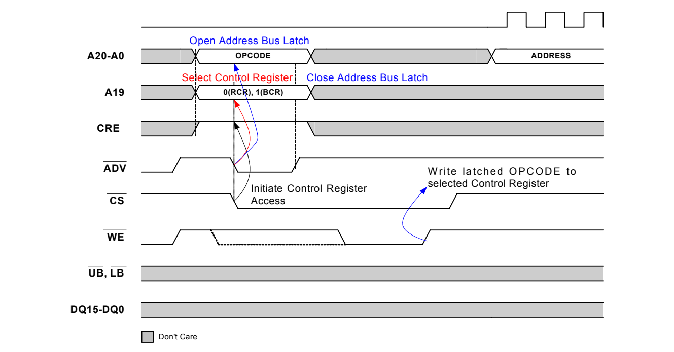
Figure 7 Control Register Write in NOR-Flash-Type Mode
