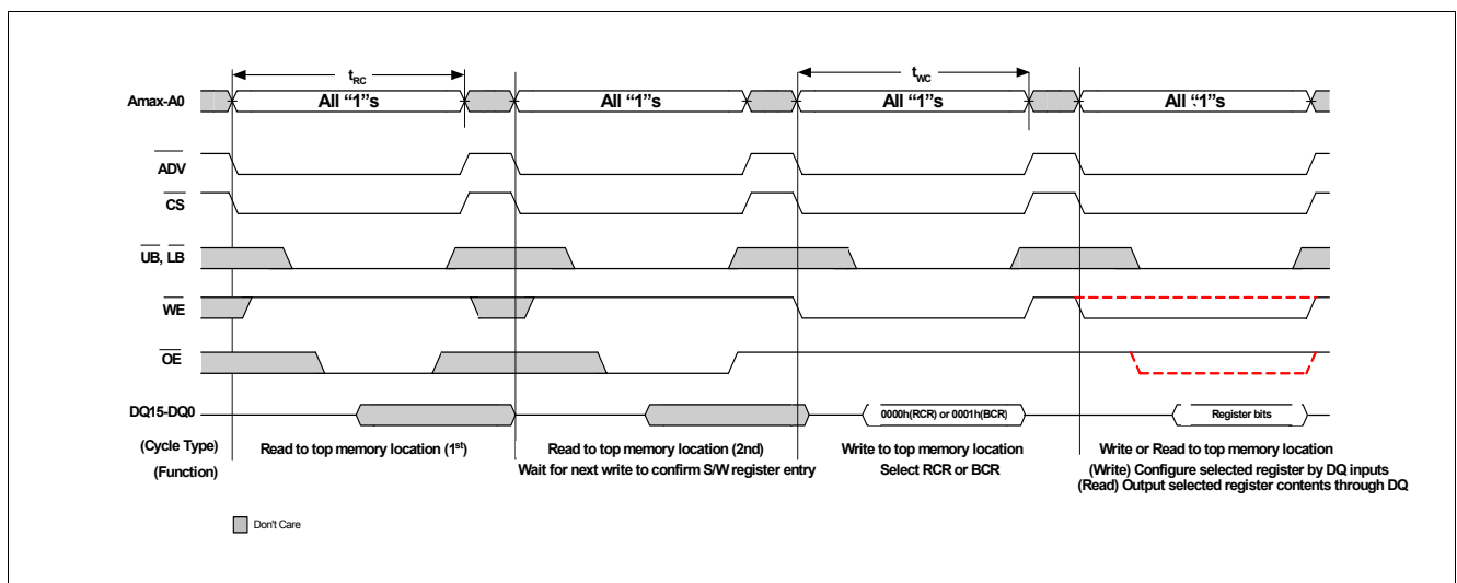
Figure 30 S/W Register Entry timing (Address input = 1FFFFh)
