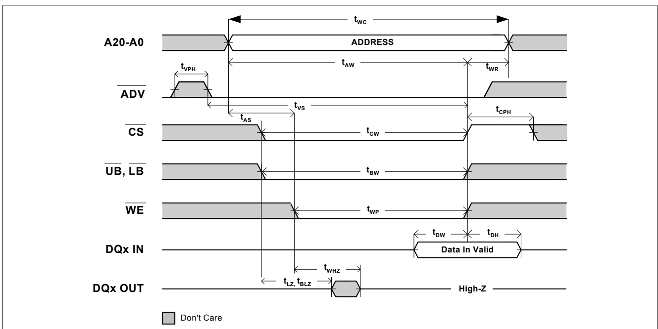
Figure 16 Asynchronous Write - \overline{CS} Controlled ( \overline{OE} = V_{IH} or V_{IL} , CRE = V_{IL} )
