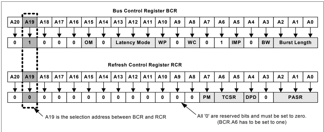
Figure 5 The two Control Registers
