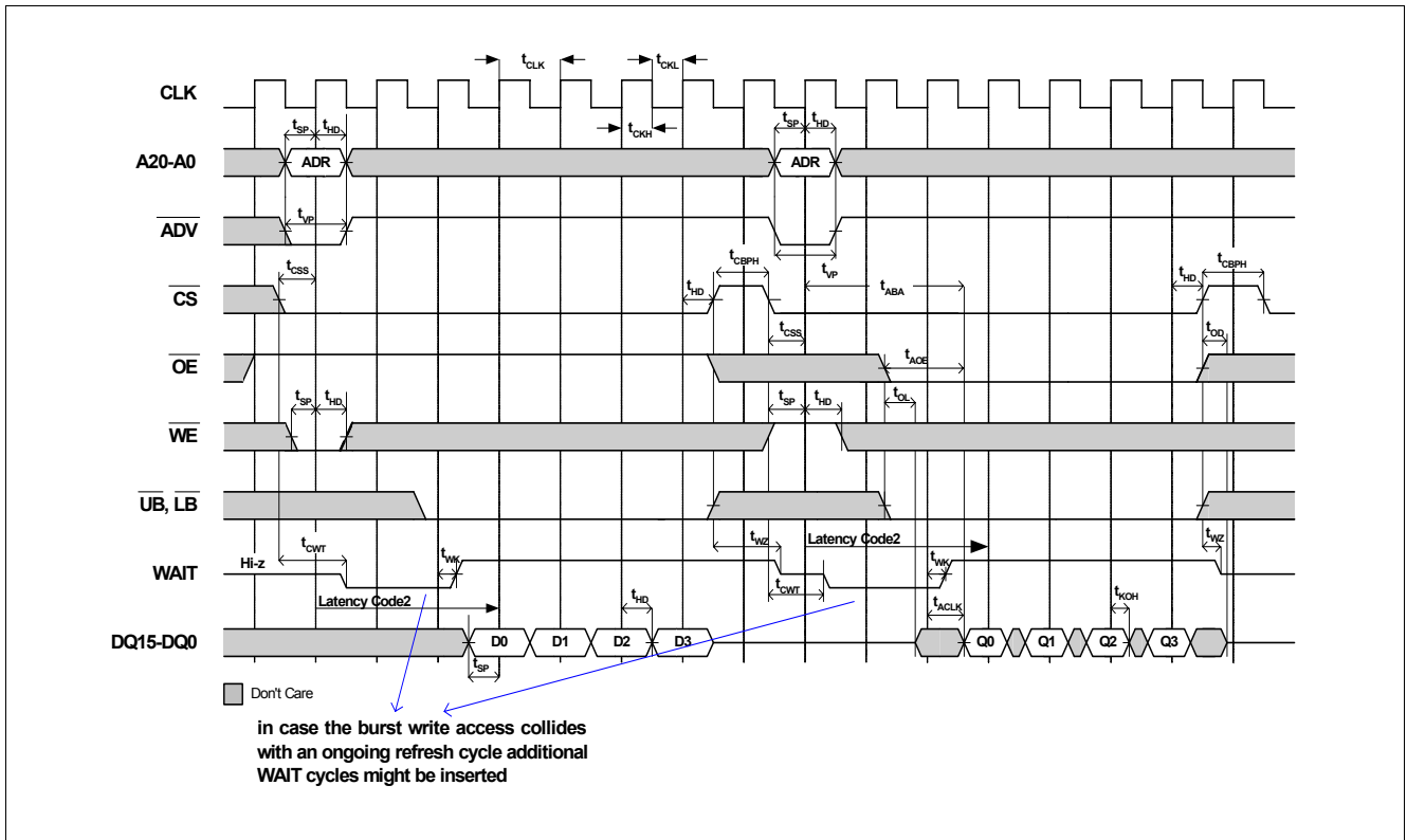
Figure 26 Synchronous Write Burst Followed by Synchronous Read Burst
