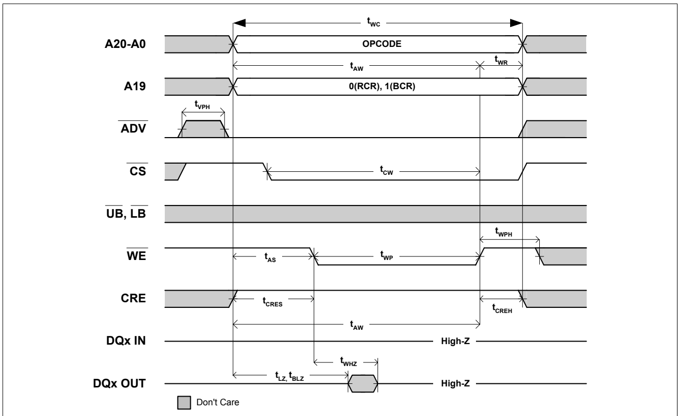
Figure 18 Asynchronous Write to Control Register ( \overline{OE} = V_{IH} or V_{IL} )
