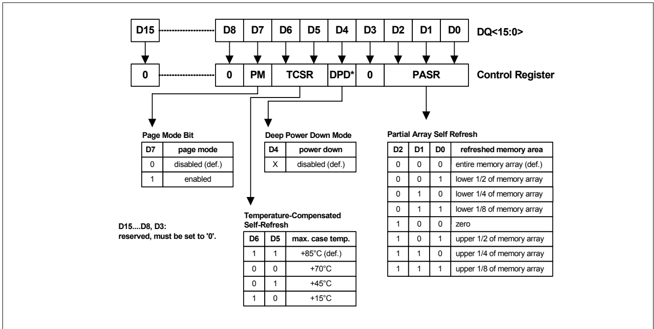
Figure 31 RCR Mapping in S/W Register Entry
