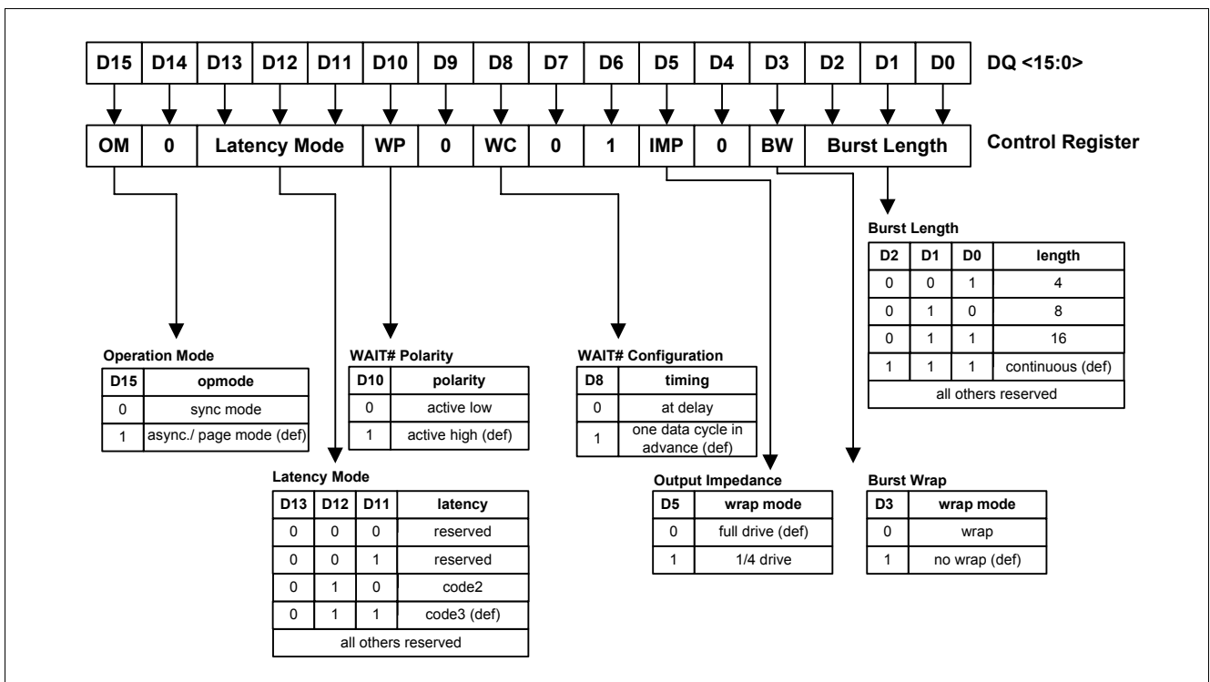
Figure 32 BCR Mapping in S/W Register Entry
