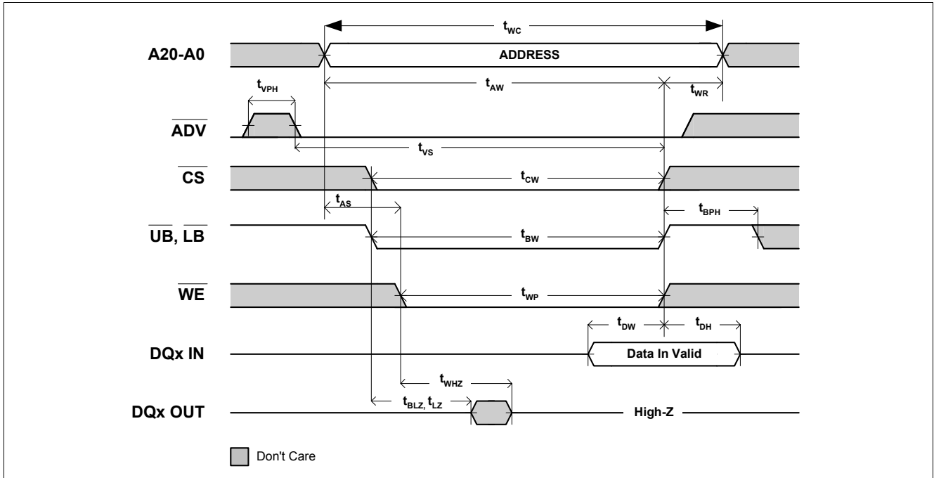
Figure 17 Asynchronous Write - \overline{UB} , \overline{LB} Controlled ( \overline{OE} = V_{IH} or V_{IL} , CRE = V_{IL} )
