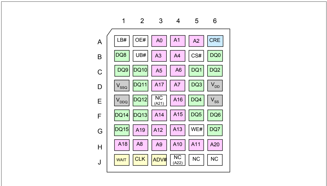
Figure 2 Standard Ballout - HYE18P32160AF-15
