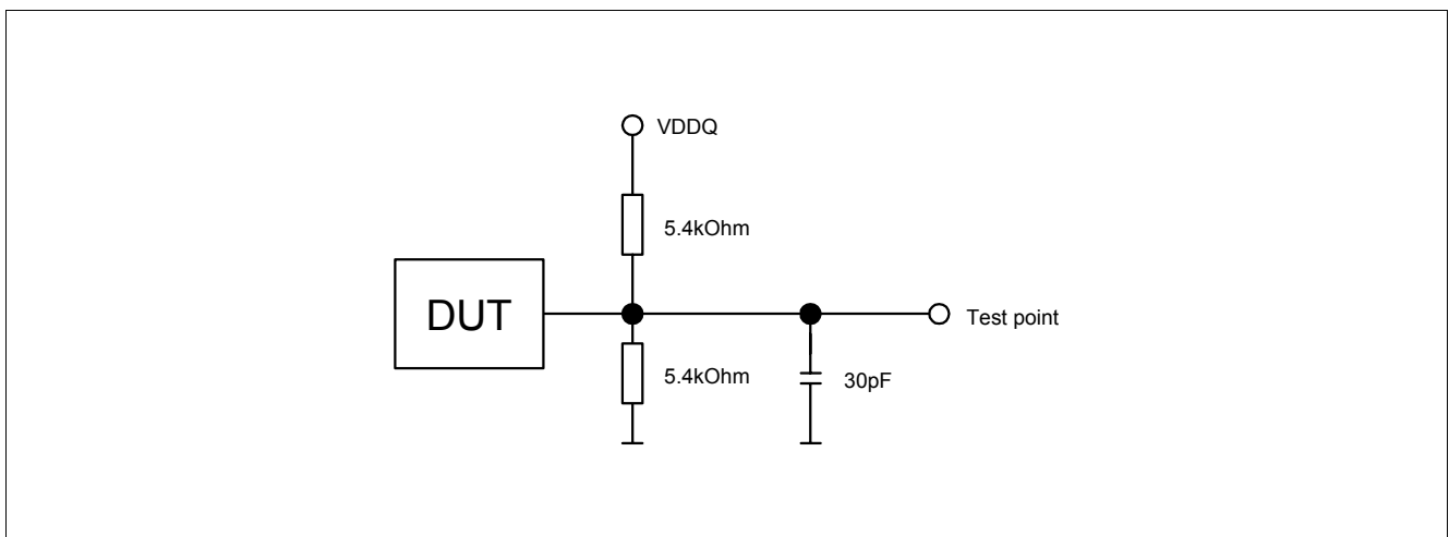
Figure 28 Output Test Circuit
