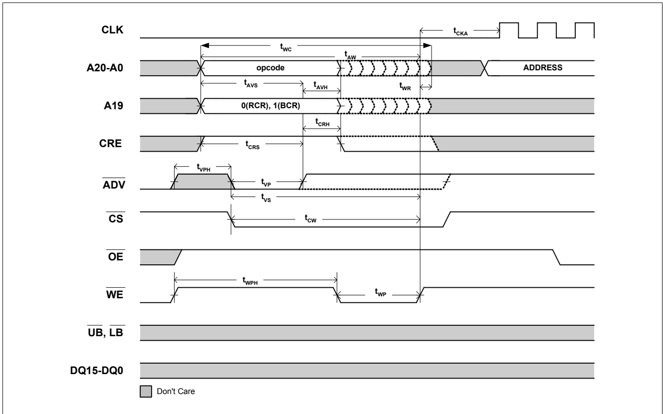
Figure 23 Asynchronous Write To Control Register in NOR-Flash Mode
