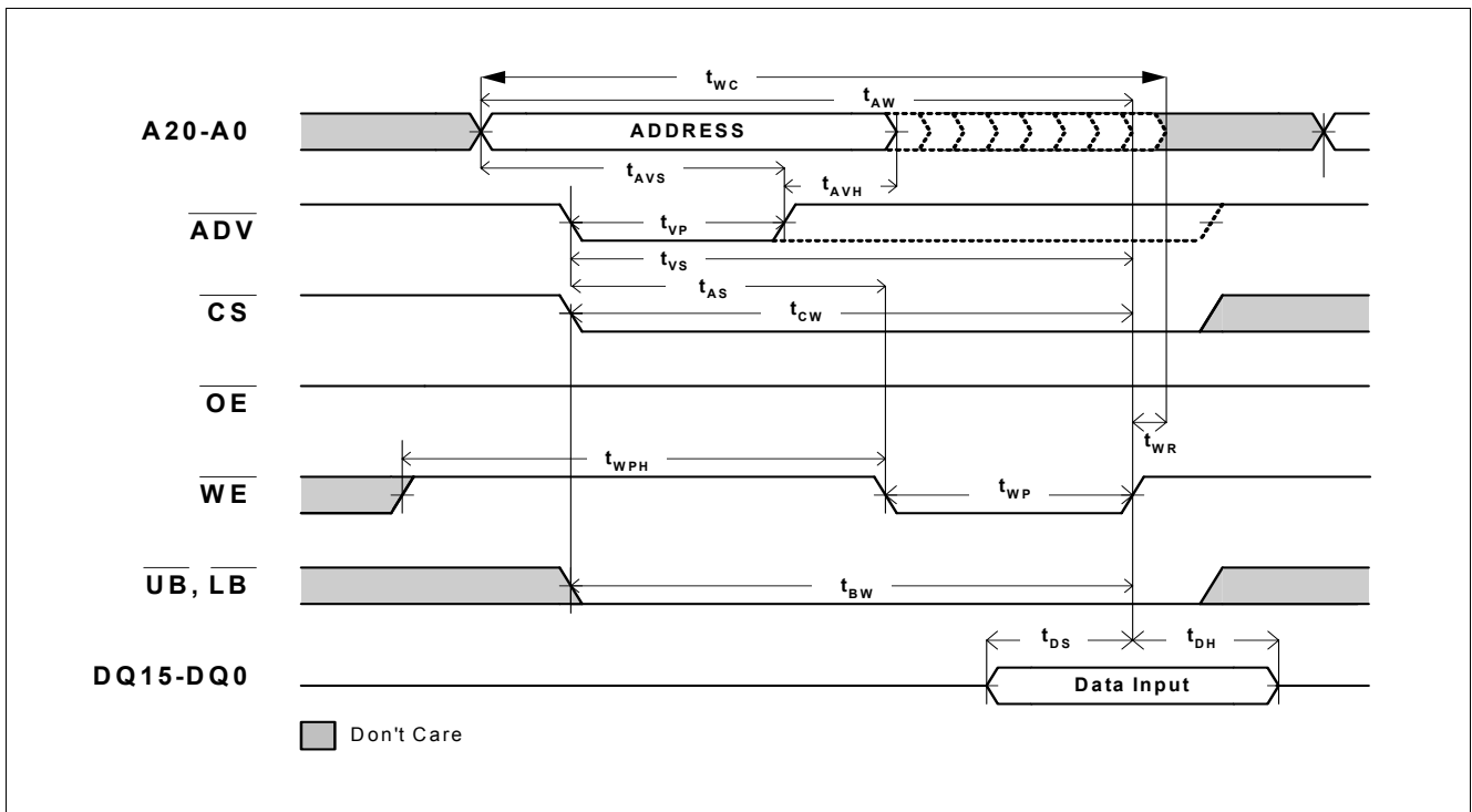
Figure 22 Asynchronous Write with Address Latch ( \overline{\text{ADV}} ) Control
