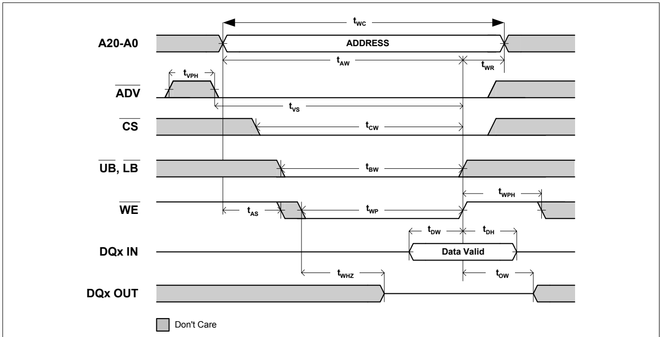
Figure 15 Asynchronous Write - \overline{WE} Controlled ( \overline{OE} = V_{IH} or V_{IL} , CRE = V_{IL} )
