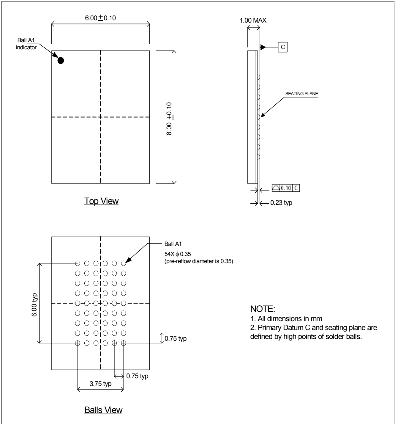
Figure 29 PG-VFBGA-54 (Plastic Very Thin Fine Pitch Ball Grid Array Package)
