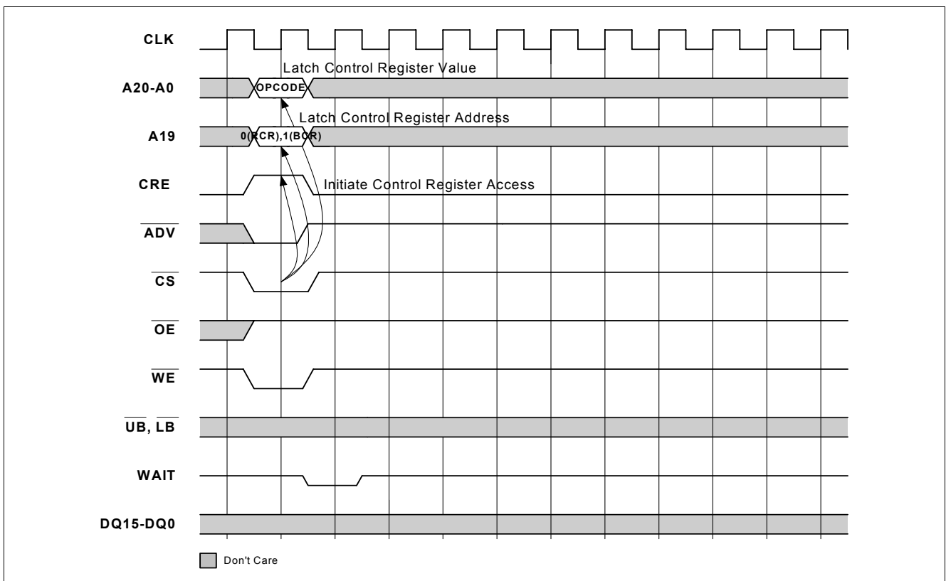
Figure 8 Control Register Write in Synchronous Mode
