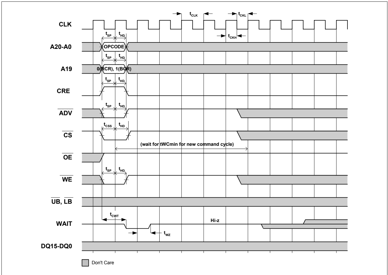
Figure 25 Synchronous Write to Control Register
