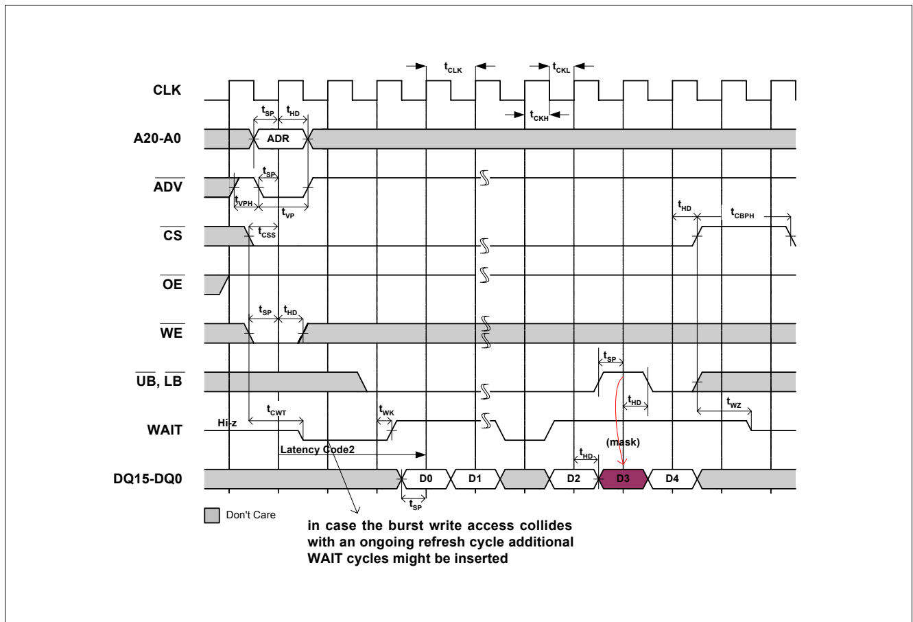
Figure 24 Synchronous Write Burst
