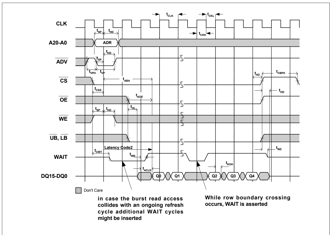
Figure 19 Synchronous Read Burst
